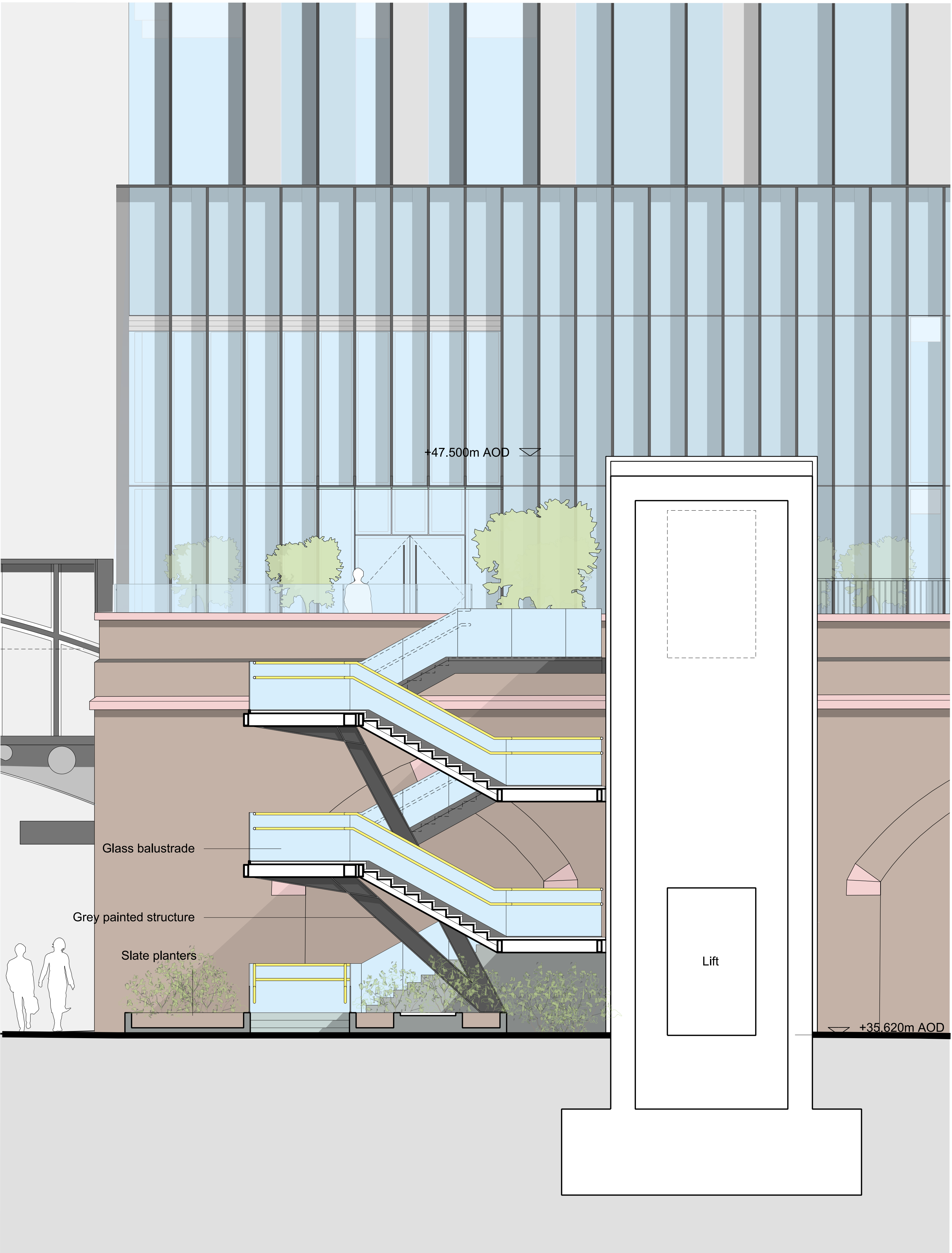
02 - Detailed Section BB
