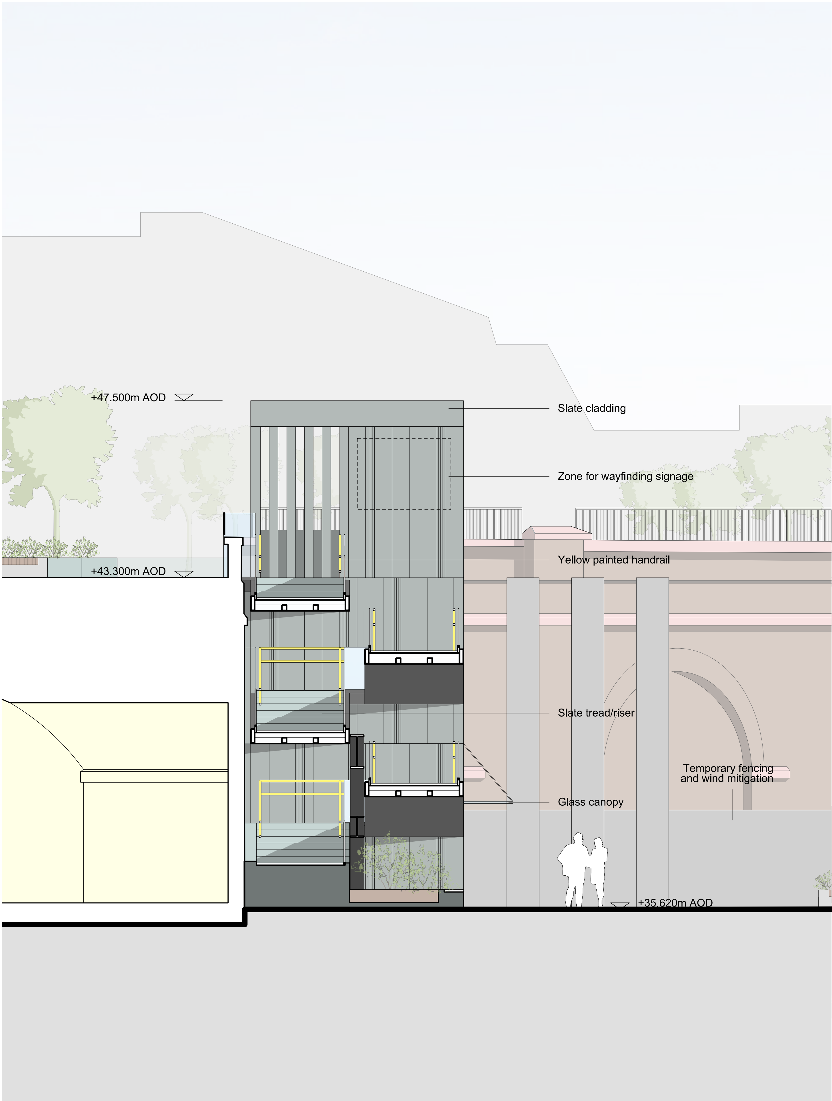
01 - Detailed Section AA
