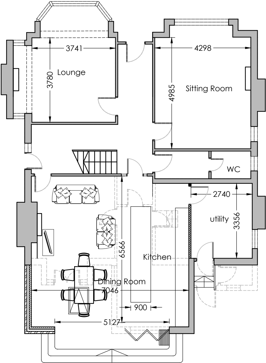
Ground Floor
