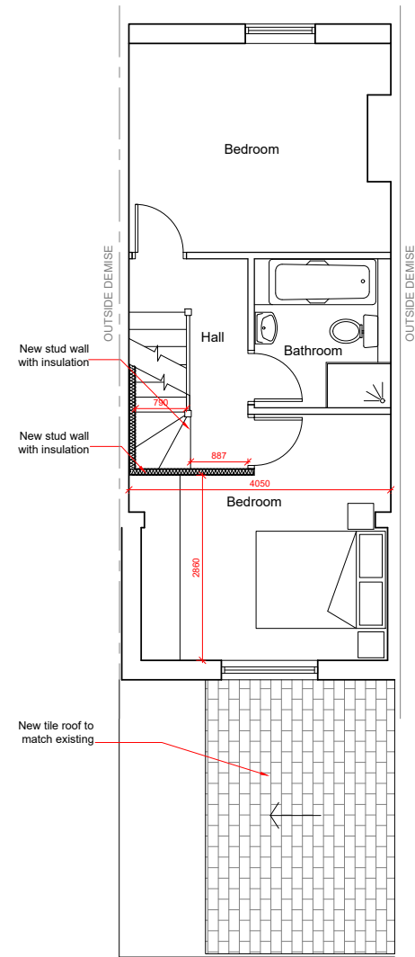
FIRST FLOOR
