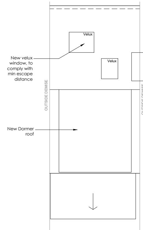
ROOF PLAN
