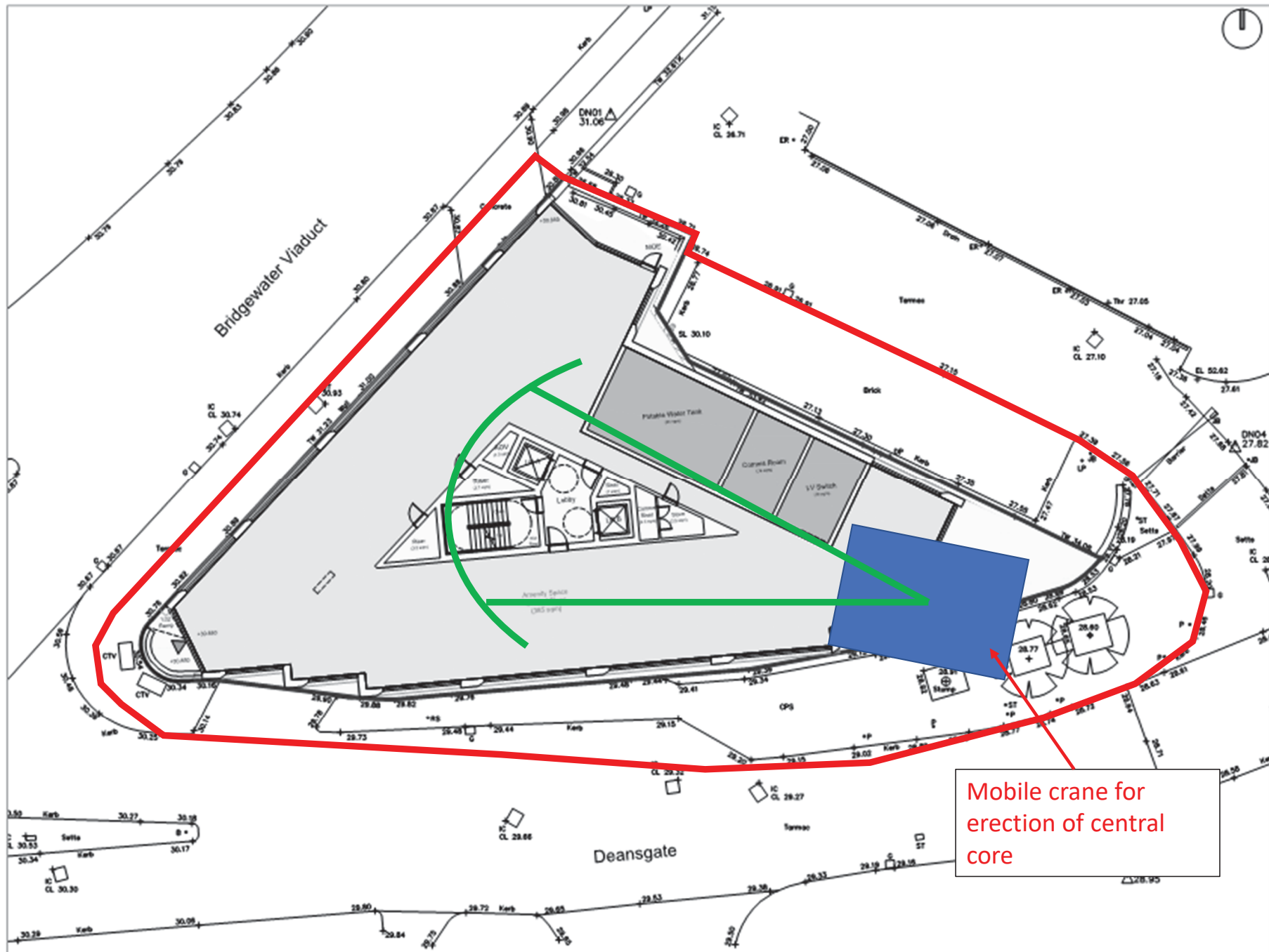
FUSION DEANSGATE – CRANEAGE STRATEGY FOR CORE
