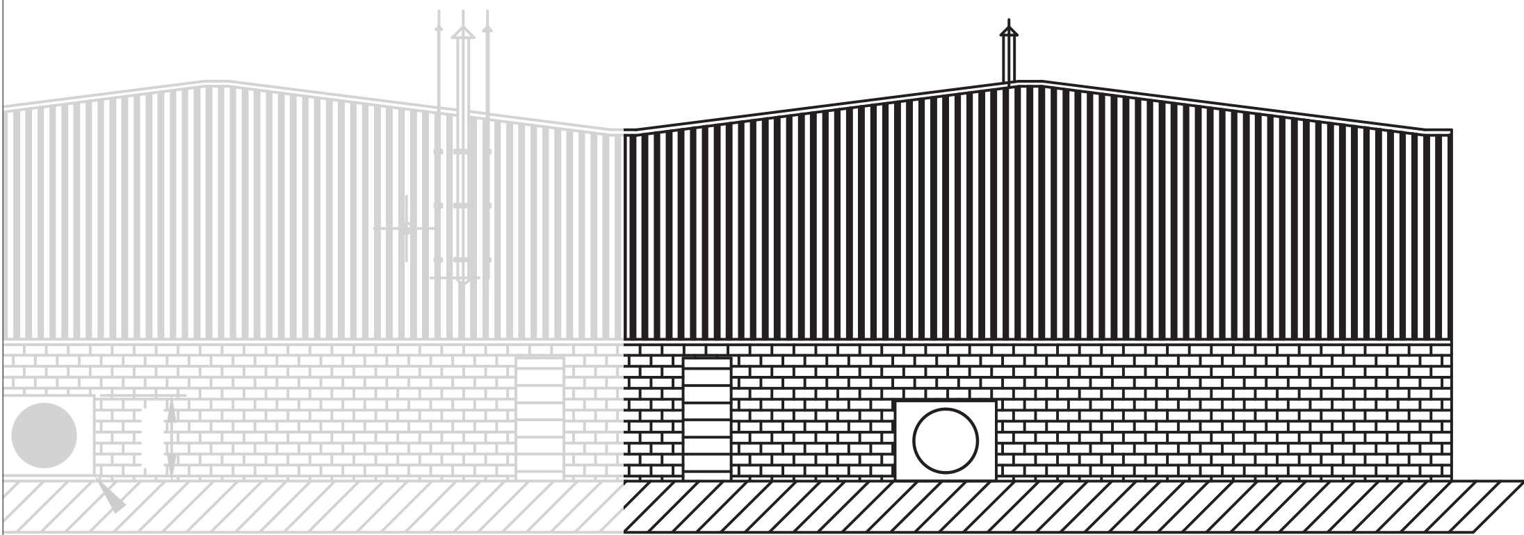
REAR ELEVATION
