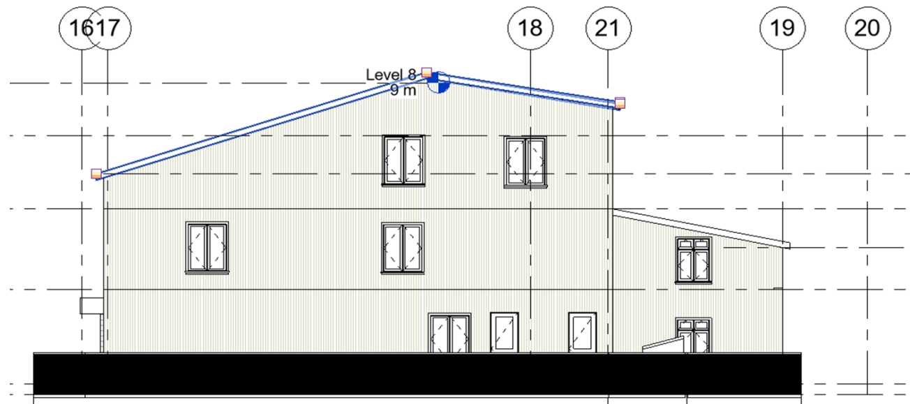
Side Elevation – Kevin Street
