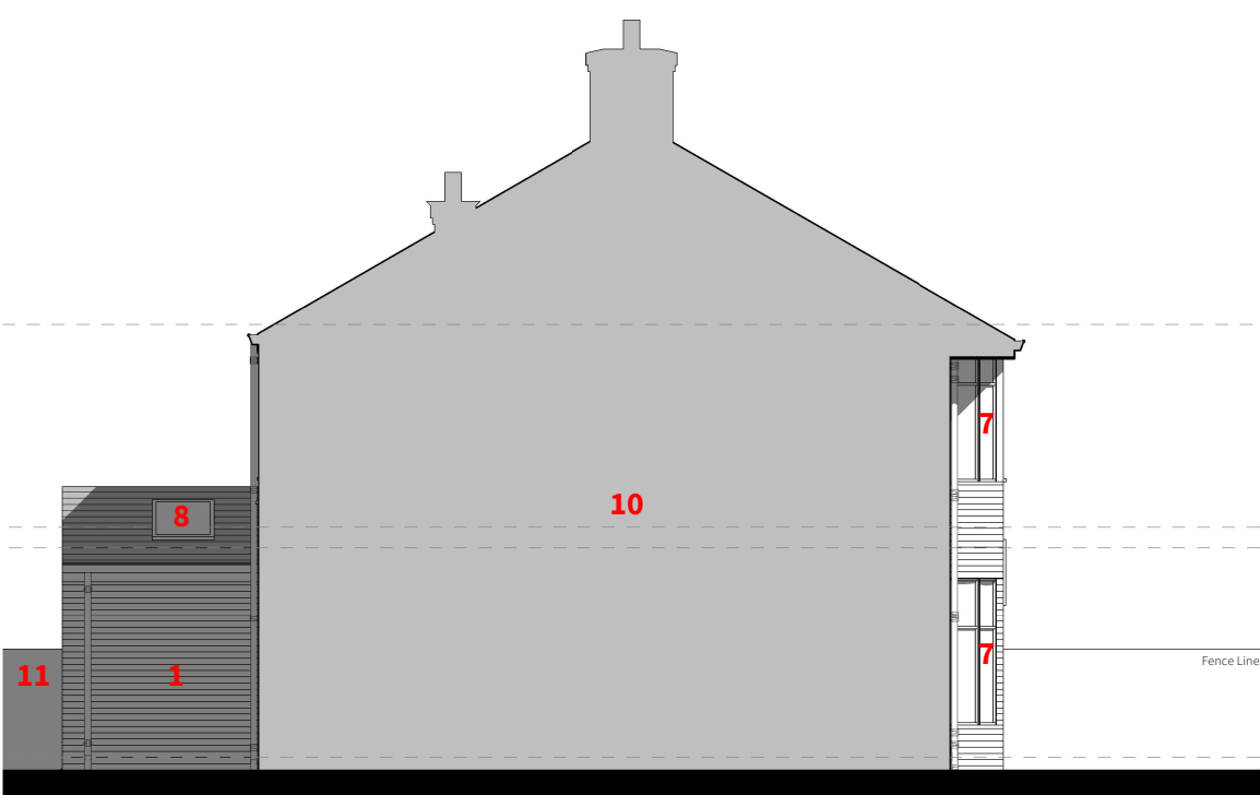
Proposed Party Wall Elevation 1:100 / A3
