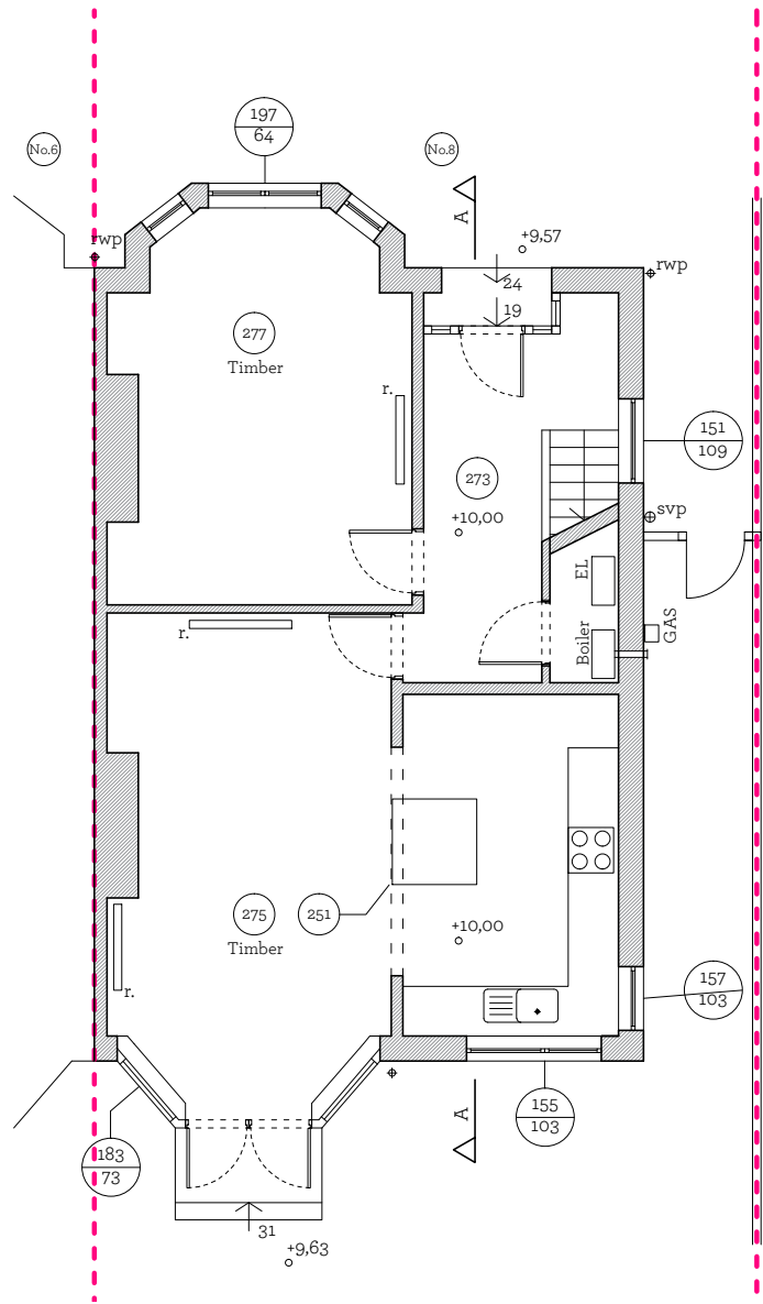
Ground Floor Plan - no change
