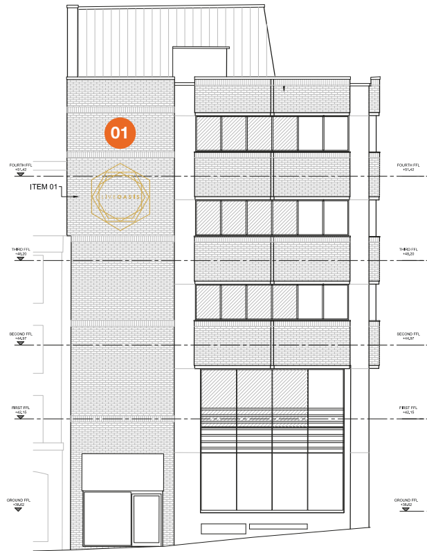
ST. JAMES SQUARE ELEVATION
