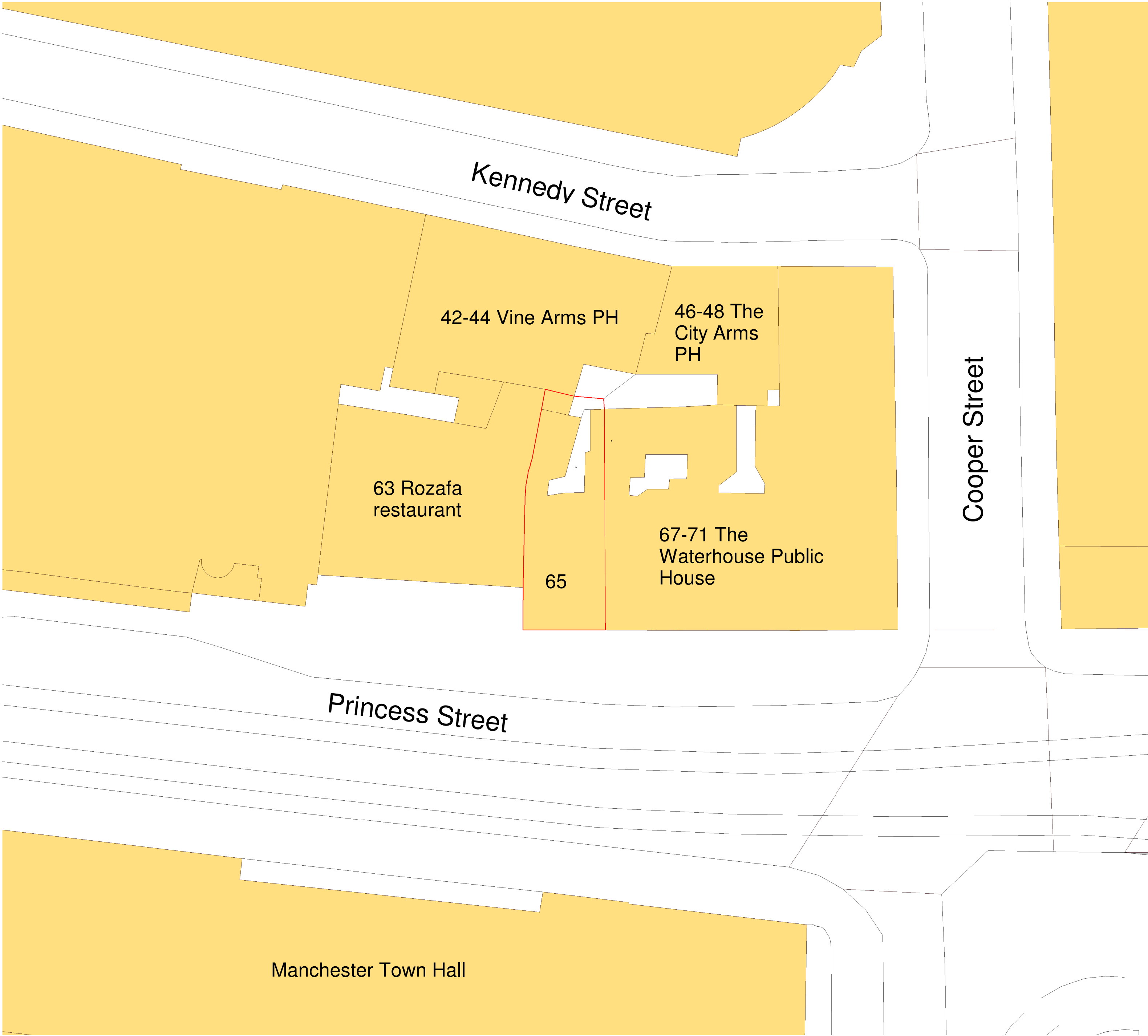
CONTEXT PLAN 1:200
