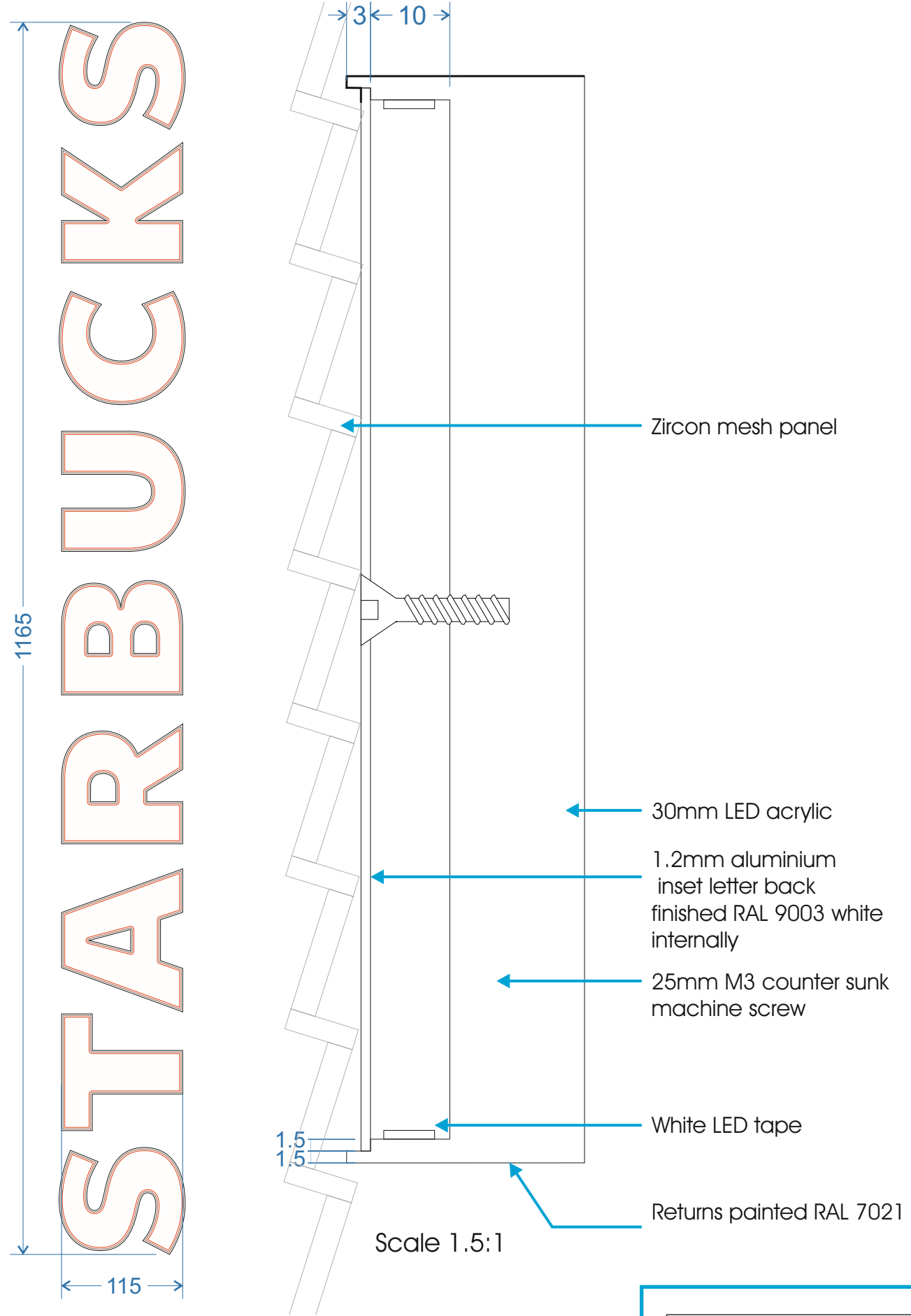
Detail B Scale 1:5
