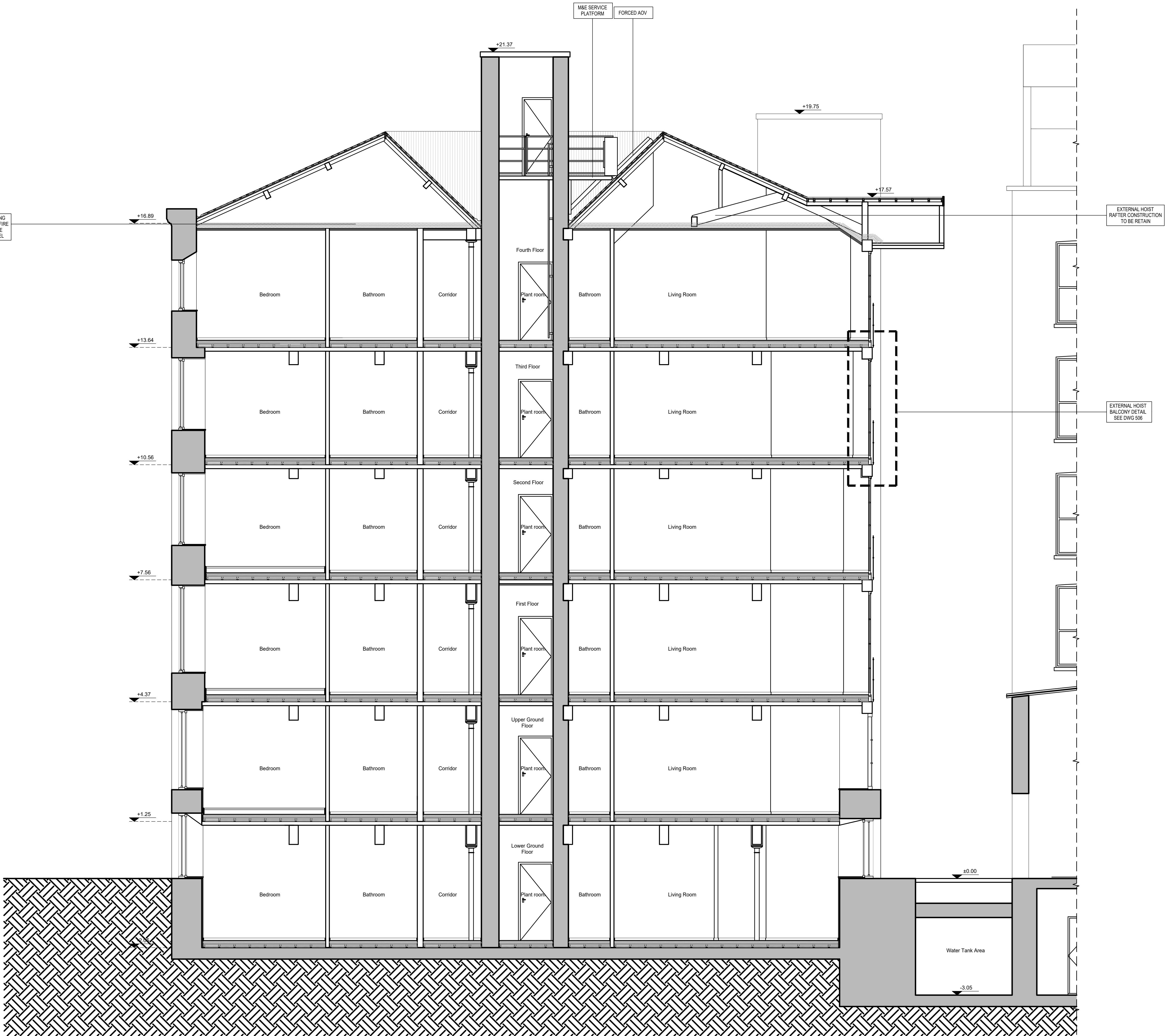
Proposed Section A-A
