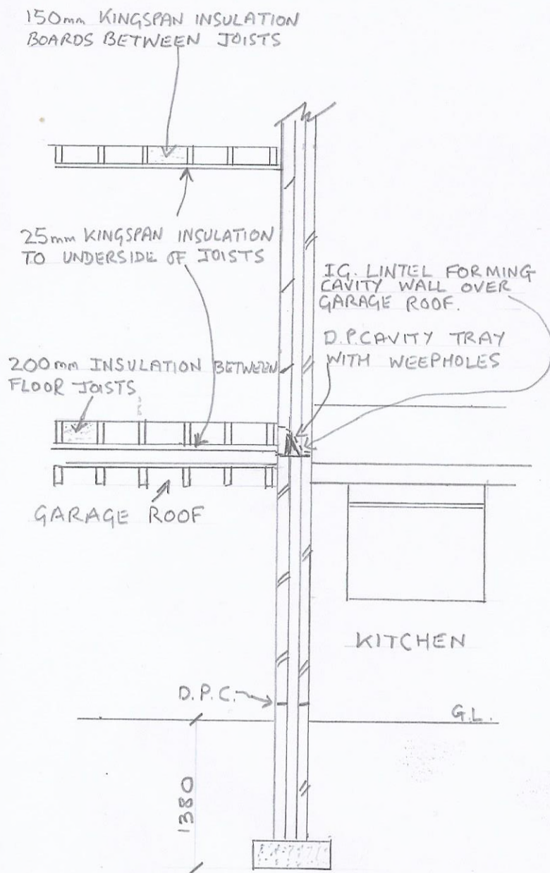
SECTION B:B
