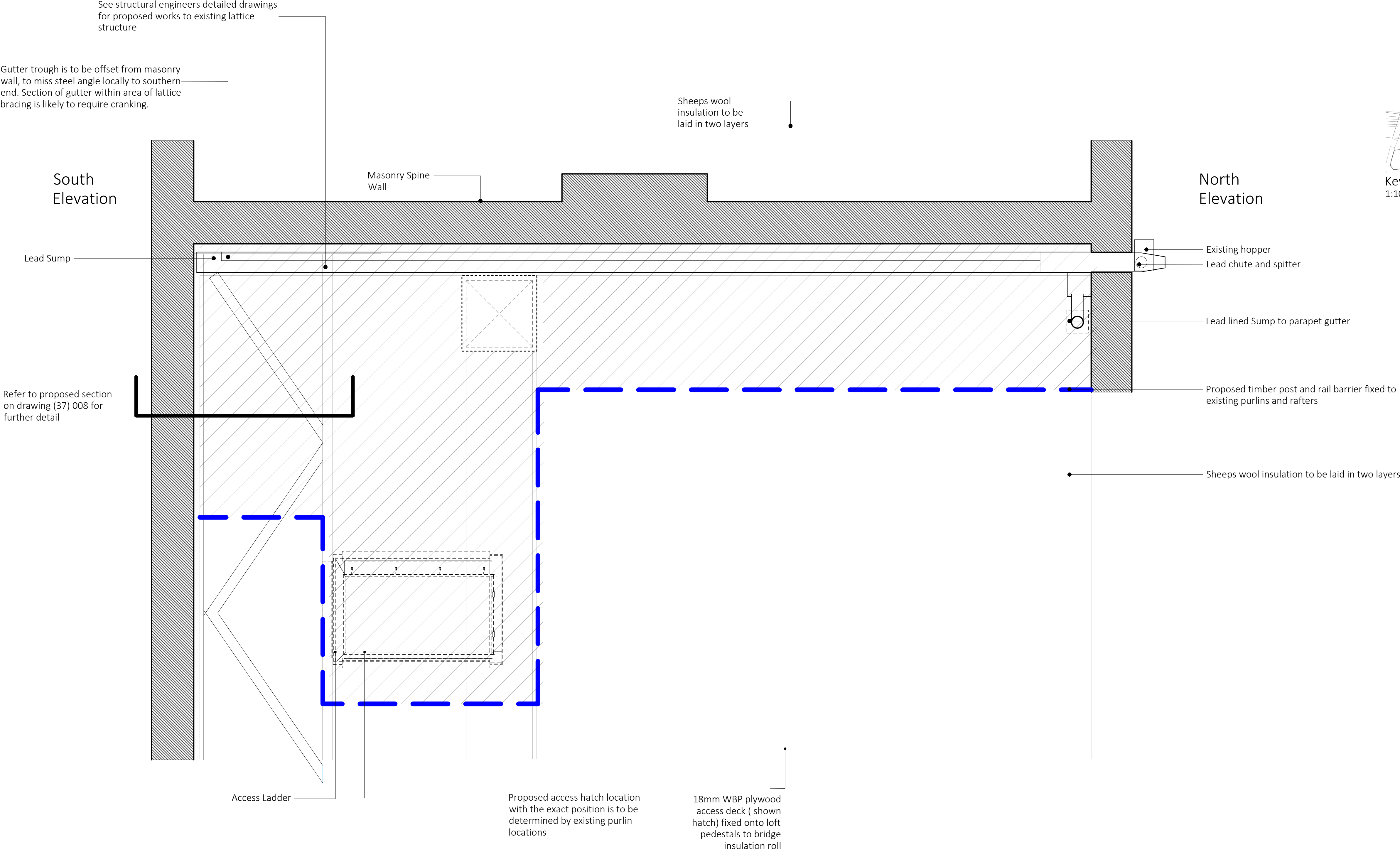
Proposed Part Attic Plan Showing Roof Access Hatch, Rooflight and Secure Internal Platform 1:20
