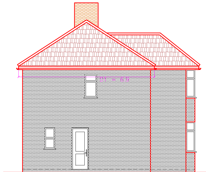
Existing Side Elevation - A
