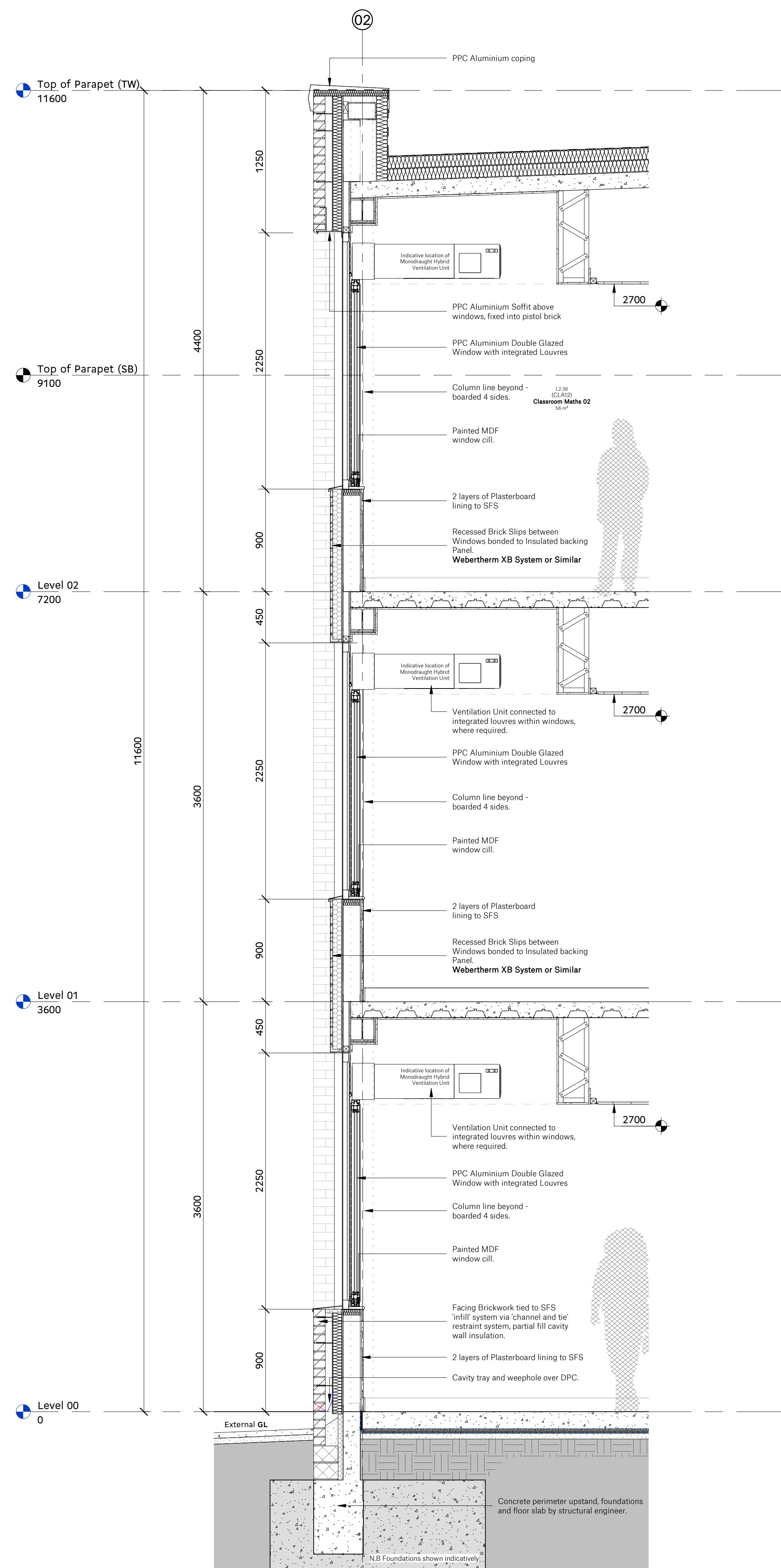
Section through Teaching Wing 1: 25
