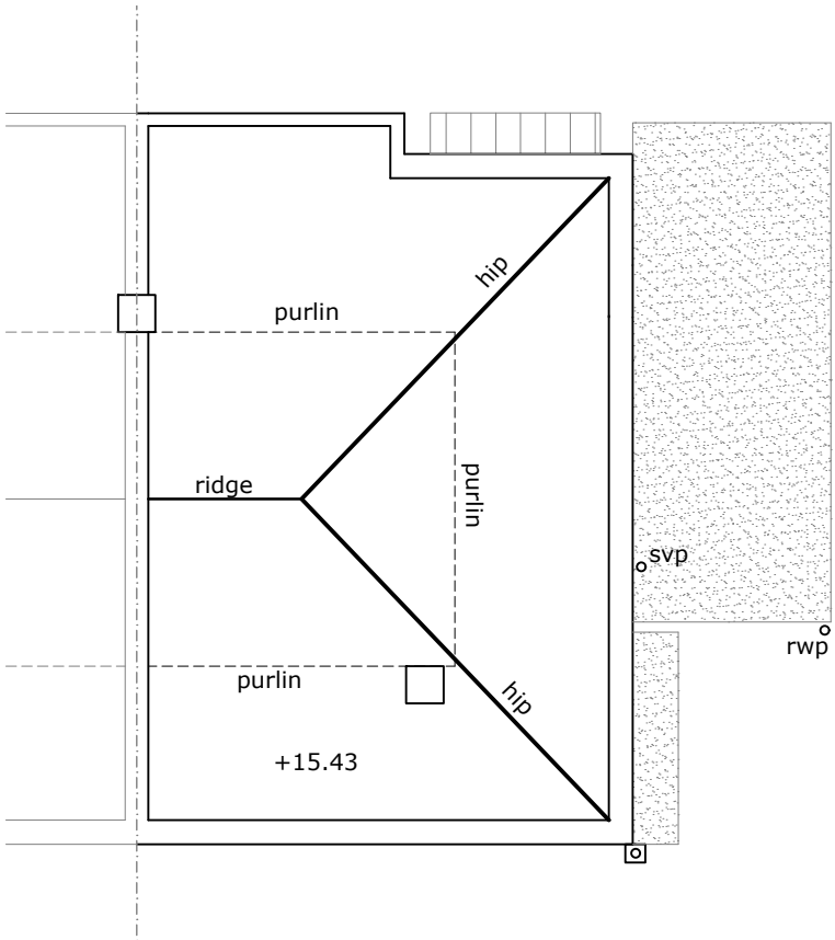
ATTIC PLAN
