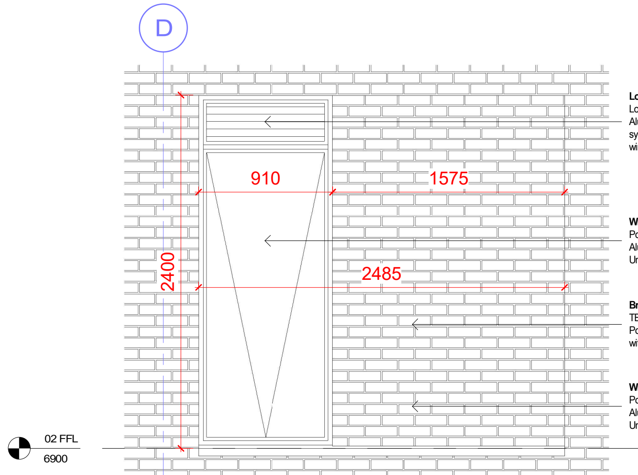
1 Recessed Window Elevation 1 : 25
