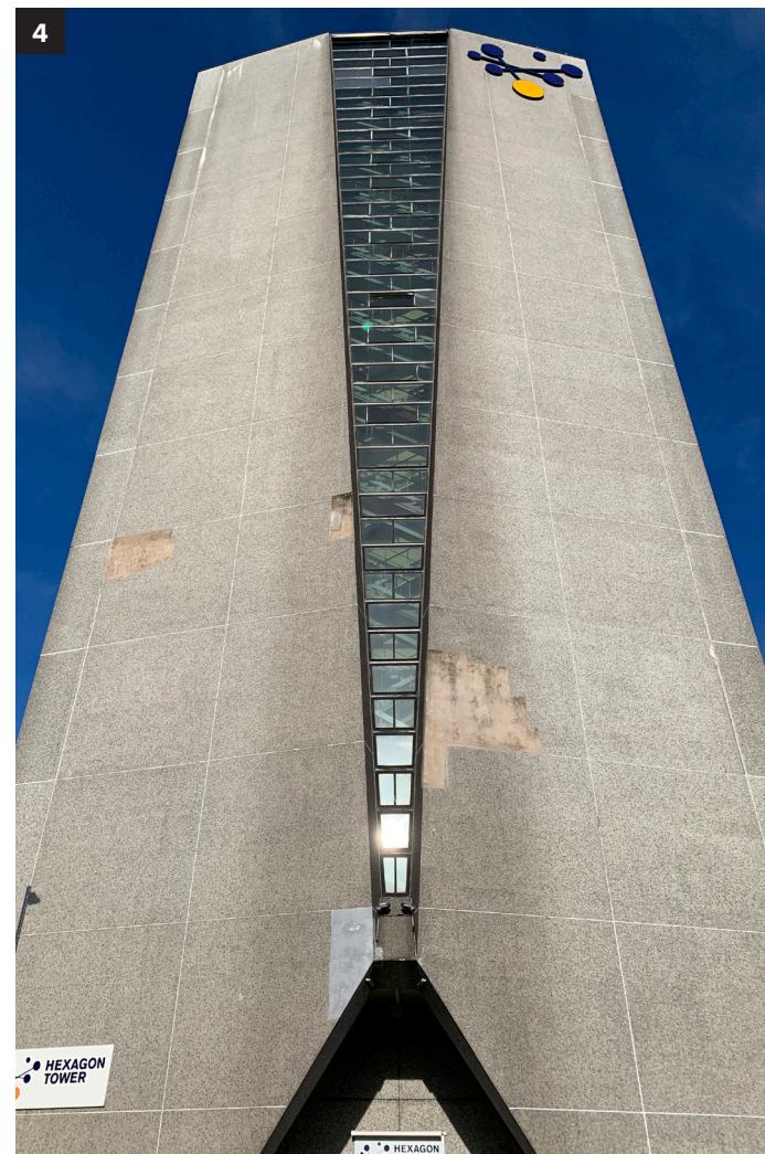
View looking up to tower; original joint lines visible; areas of mosaic delamination and remediation apparent.
