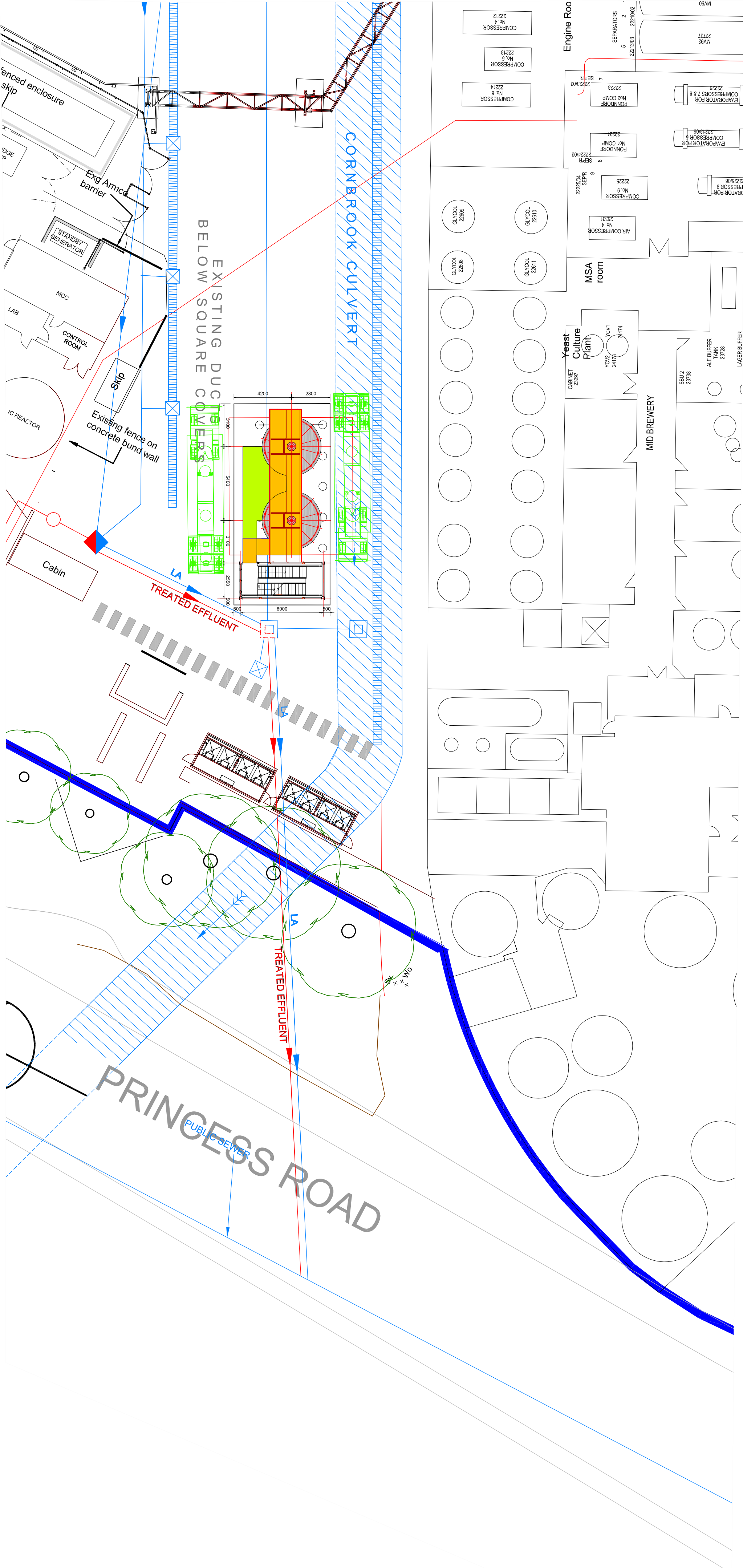
SITE BLOCK PLAN - GROUND FLOOR LEVEL
