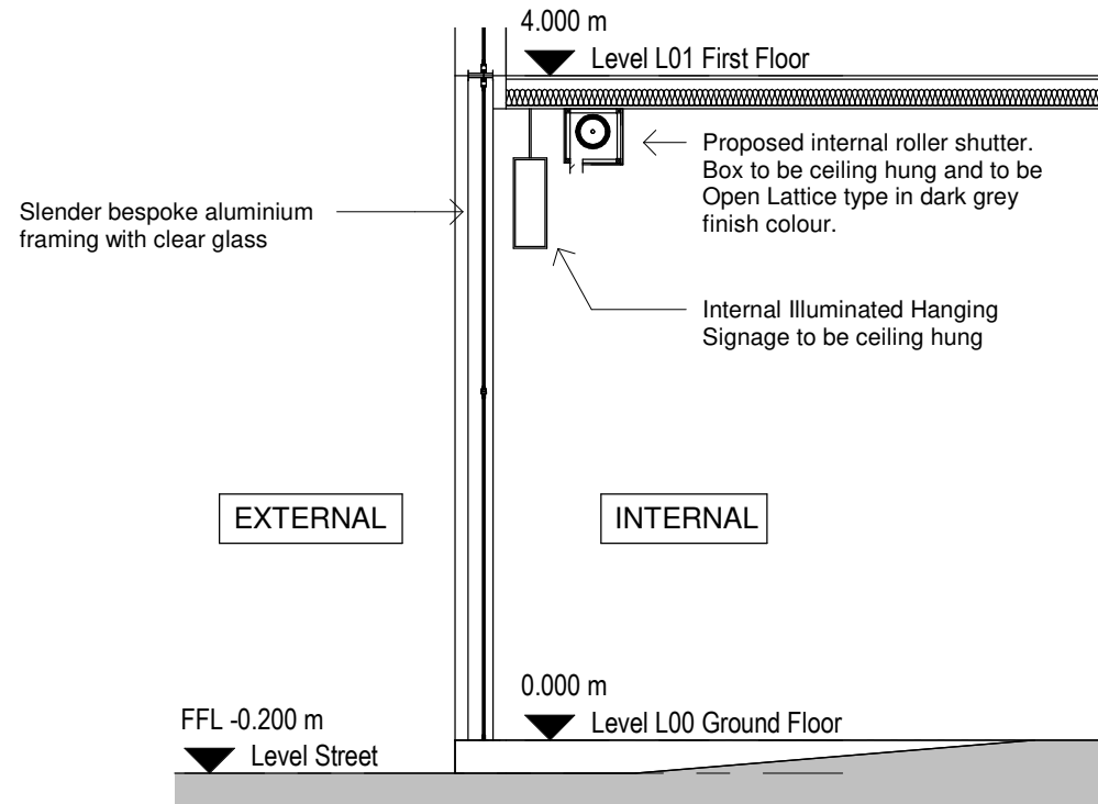
2 Shop Front Section 1 : 50
