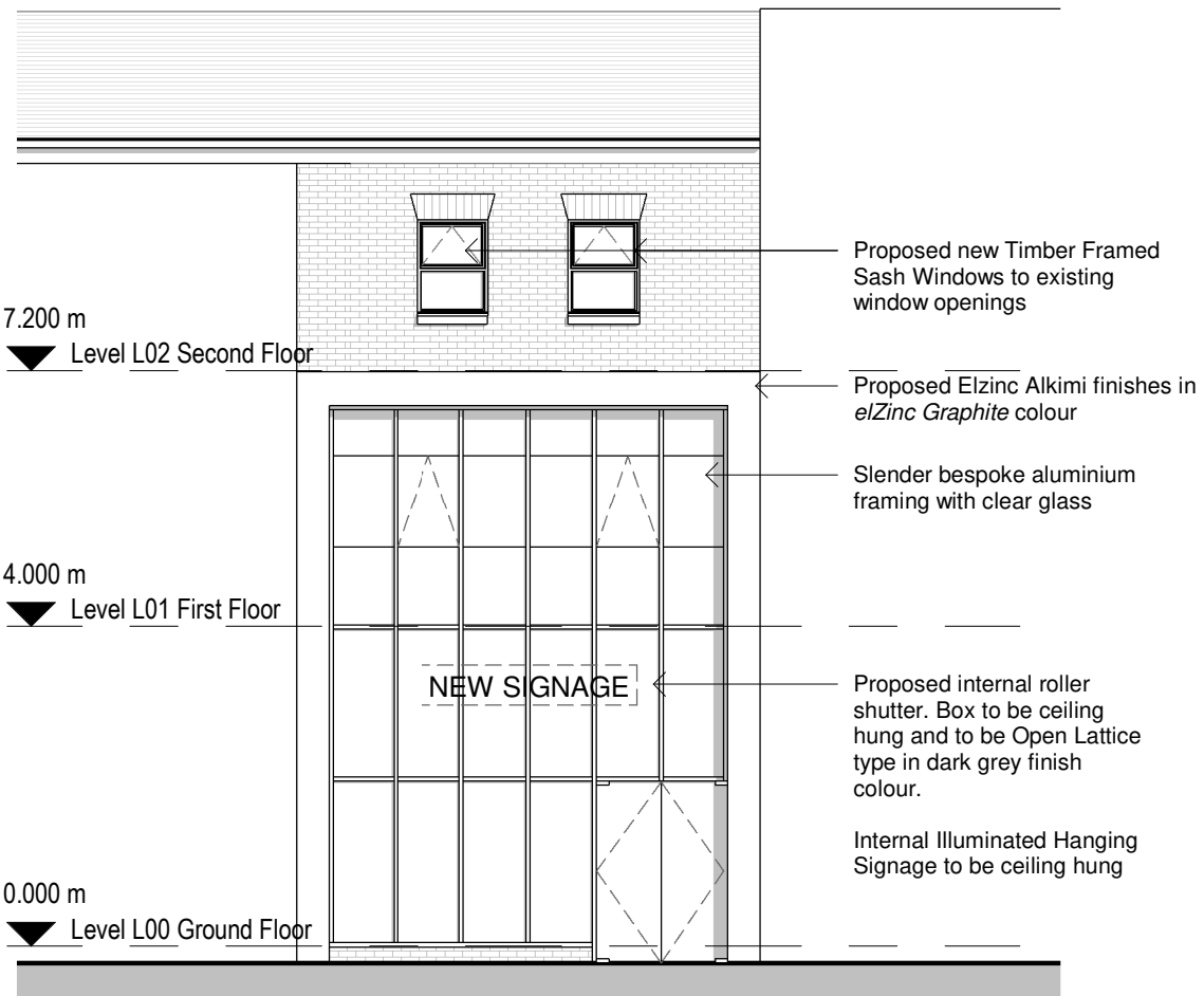
1 Proposed West Elevation 1 : 100
