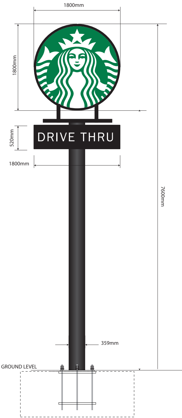
Rear Elevation
