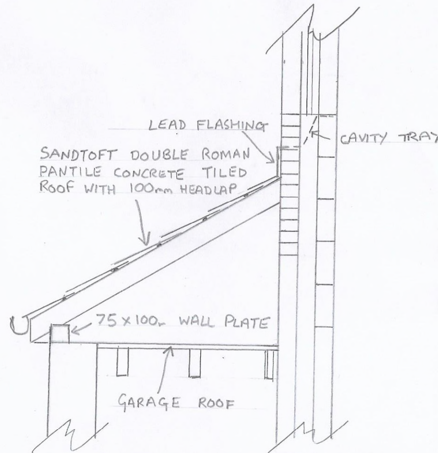
DETAIL A SCALE 1:20
