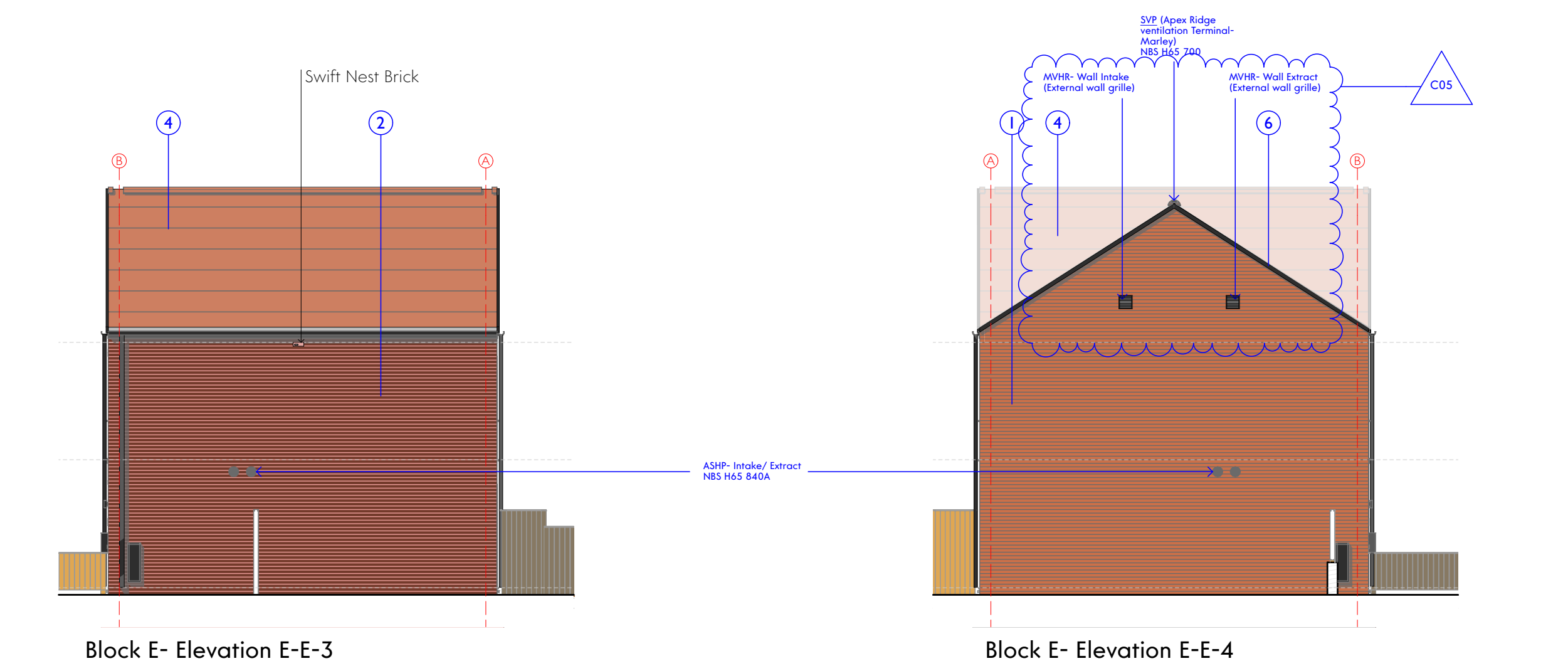
Block E- Elevation E-E-3
