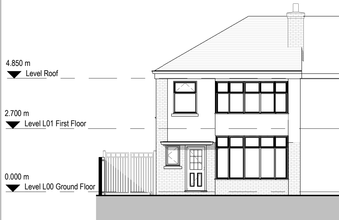
1 Existing East Elevation 1 : 100
