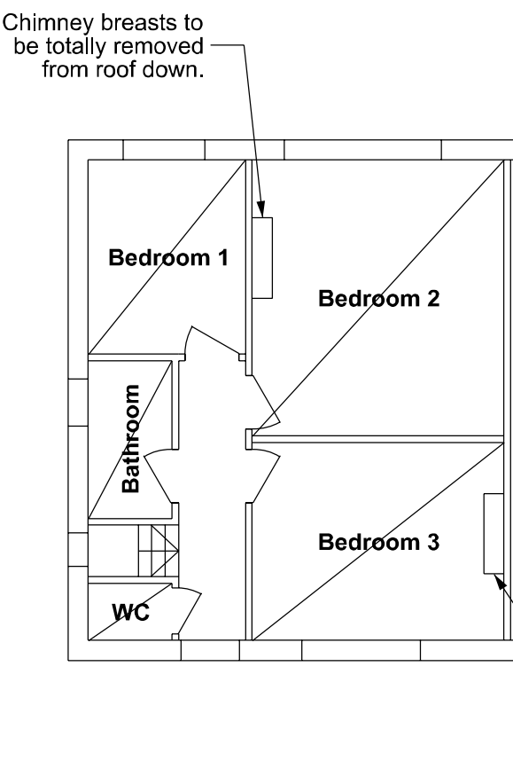
Existing First Plan
