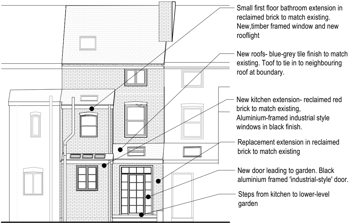
Rear Elevation (East) 1:100@A3
