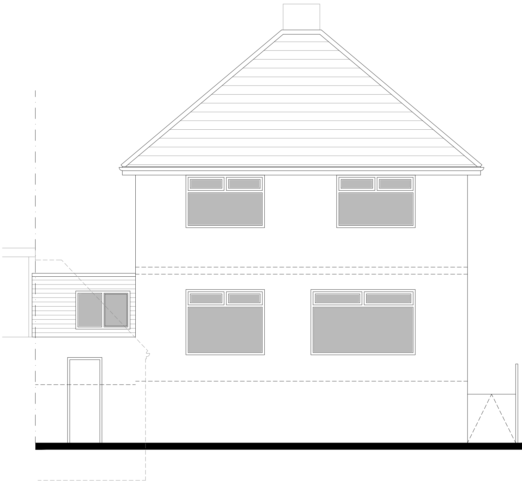
rear elevation
