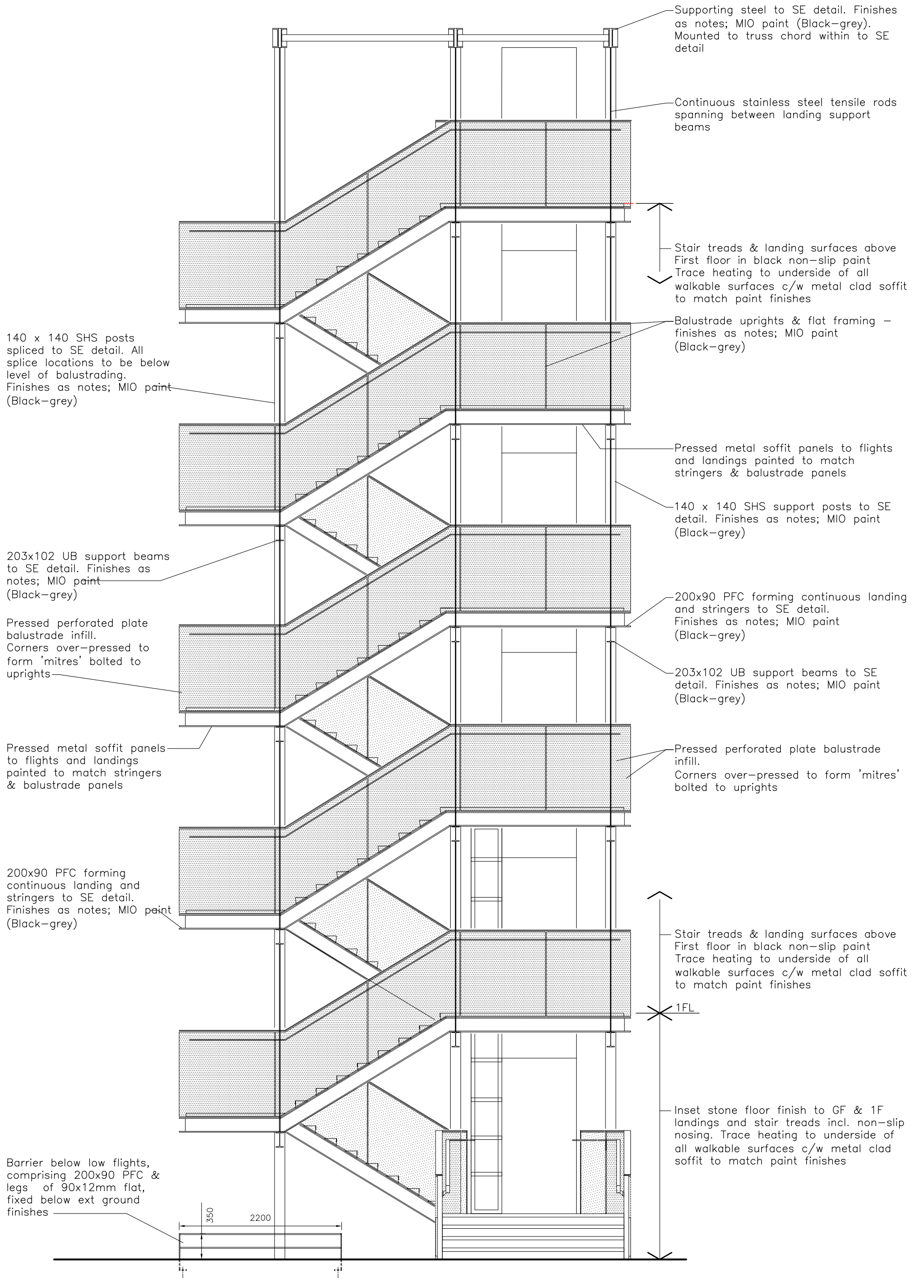
ELEVATION TO Gt ANCOATS St.
