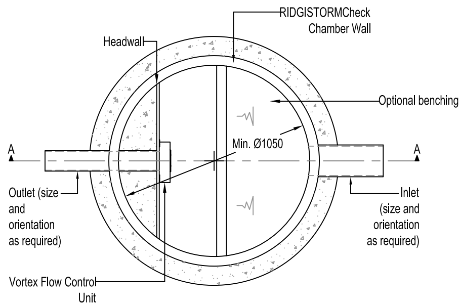
PLAN VIEW Scale (1:30)
