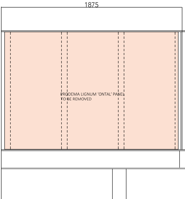
02. SIDE ELEVATION
