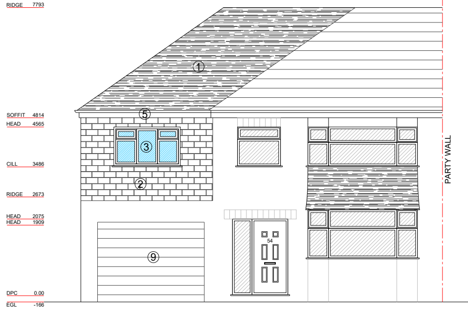
FRONT ELEVATION
