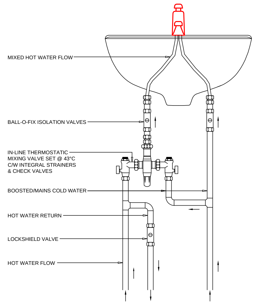
TYPICAL BLENDED HOT WATER PIPEWORK ARRANGEMENT (ONLY APPLICABLE ON WHB'S & SINKS WITH NON-THERMOSTATIC TAPS)
