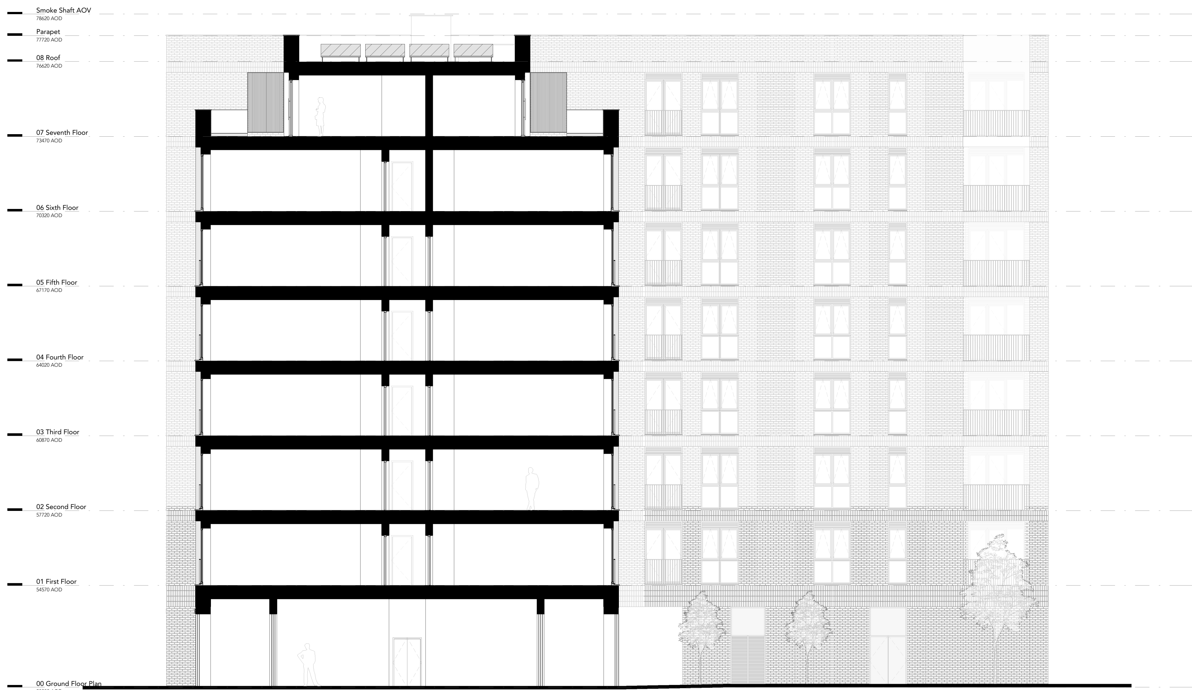
Section 2-2 1:100
