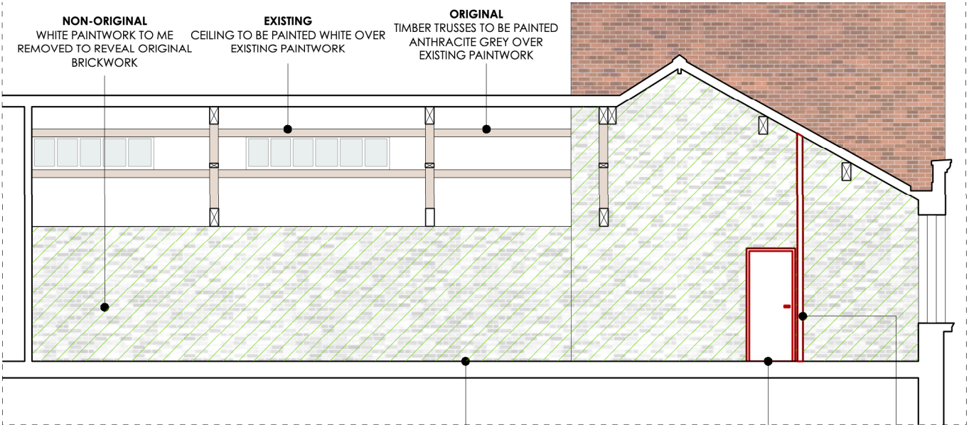
FOURWAYS HOUSE, FIFTH FLOOR ALTERATIONS SECTION DD'
