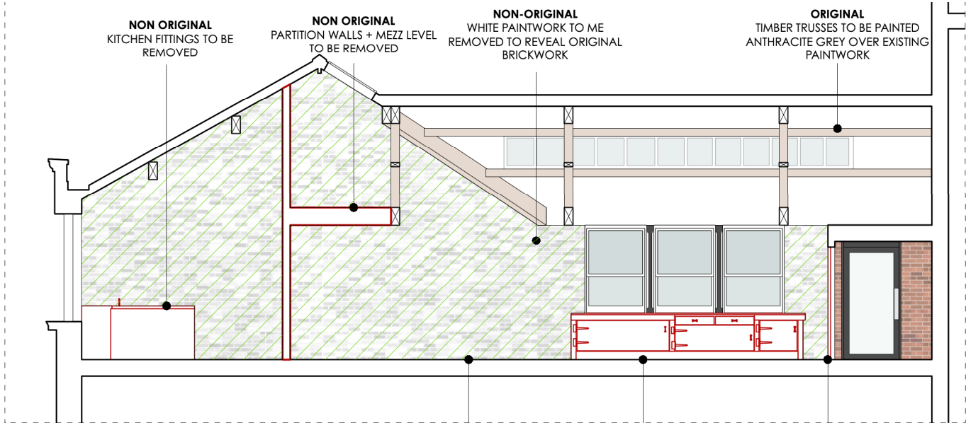
FOURWAYS HOUSE, FIFTH FLOOR ALTERATIONS SECTION CC'
