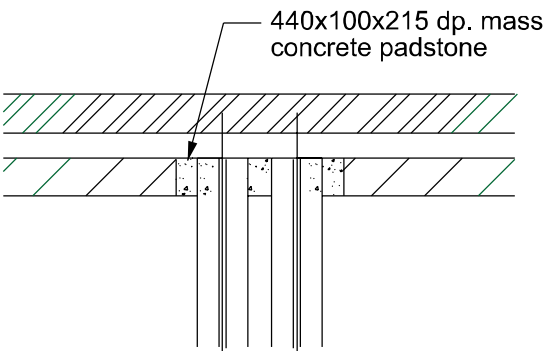
Plan on Typical Beam Bearing Detail
