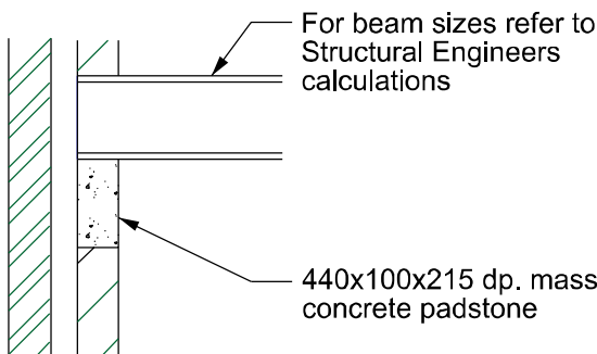
Section Thro' Typical Beam Bearing Detail
