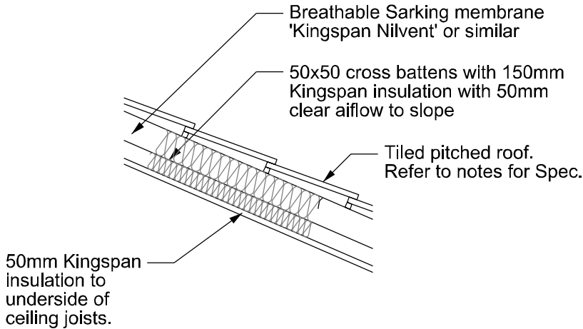
Sloping Roof Insulation Detail
