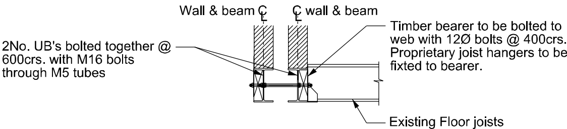
Cavity Wall Beam Support Detail
