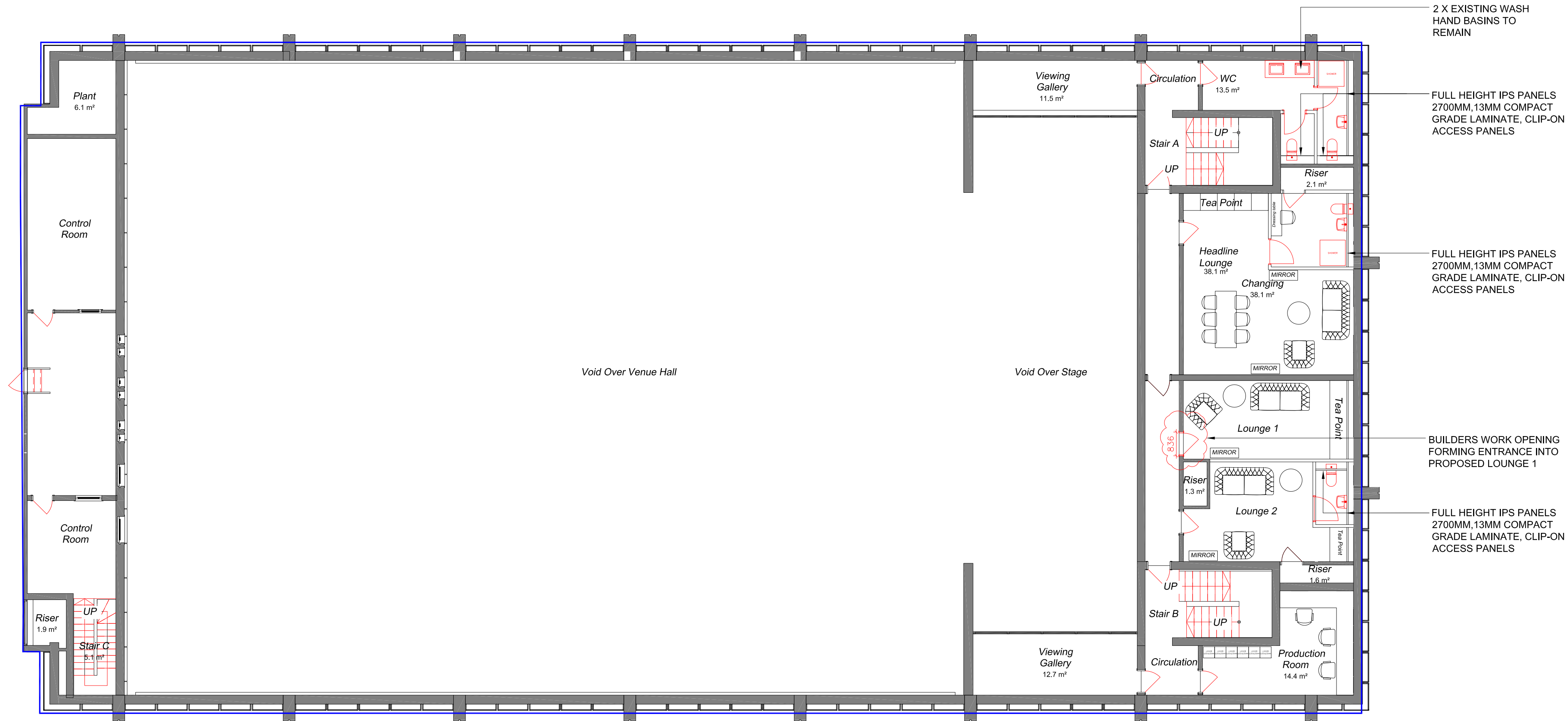
01 MEZZANINE GENERAL ARRANGEMENT PLAN Scale 1:100
