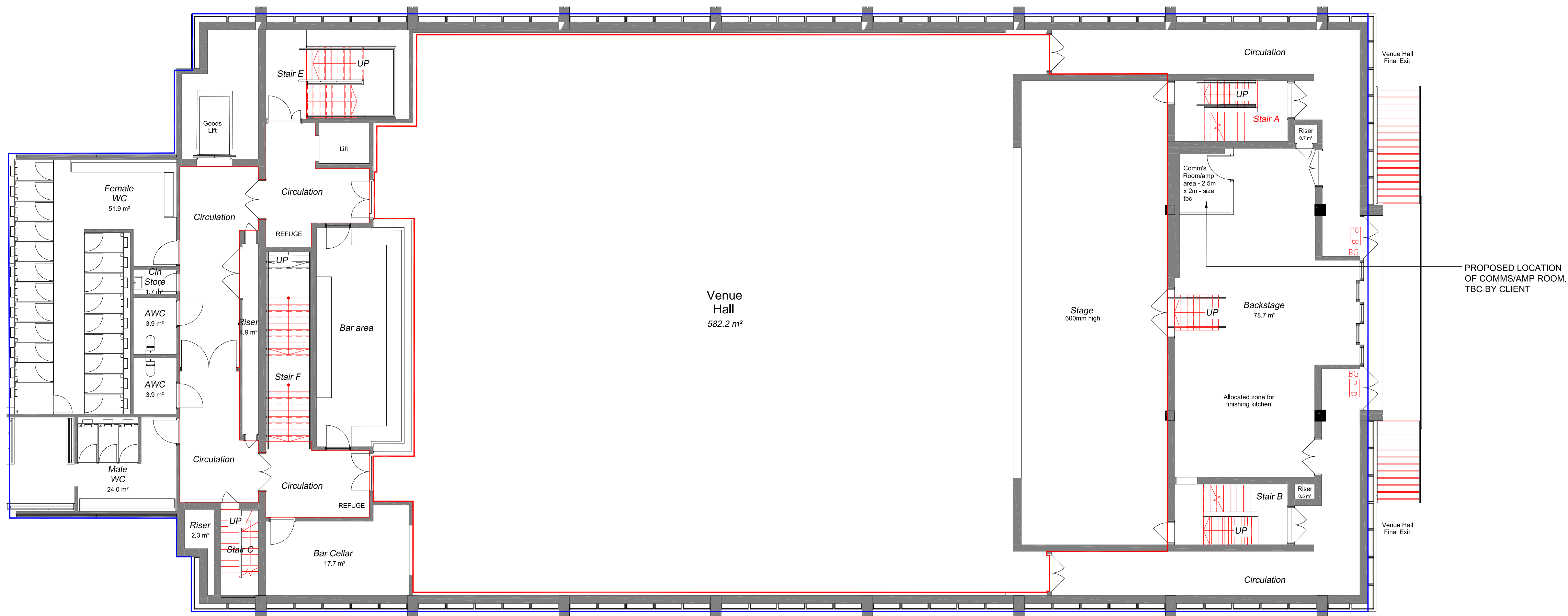
01 MEZZANINE GENERAL ARRANGEMENT PLAN Scale 1:100
