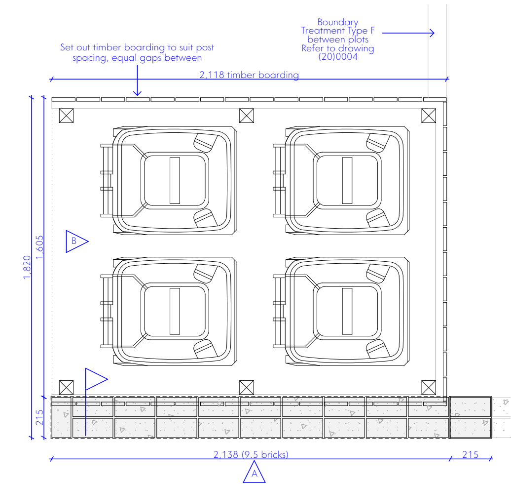
Timber fencing setting out plan
