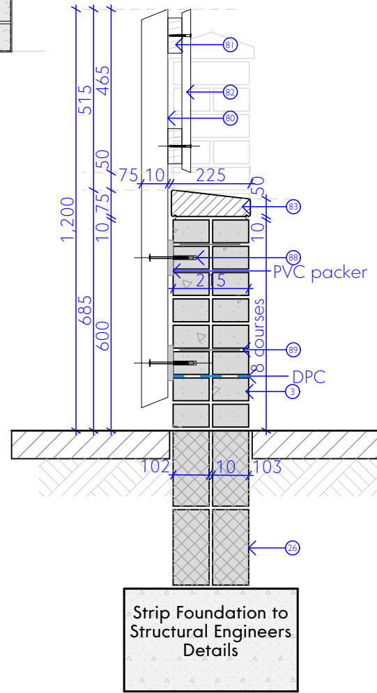
Typical section detail
