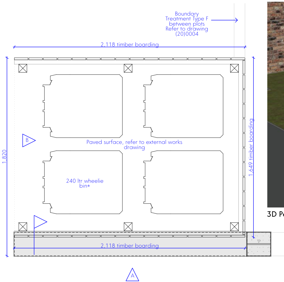
Timber fencing setting out plan
