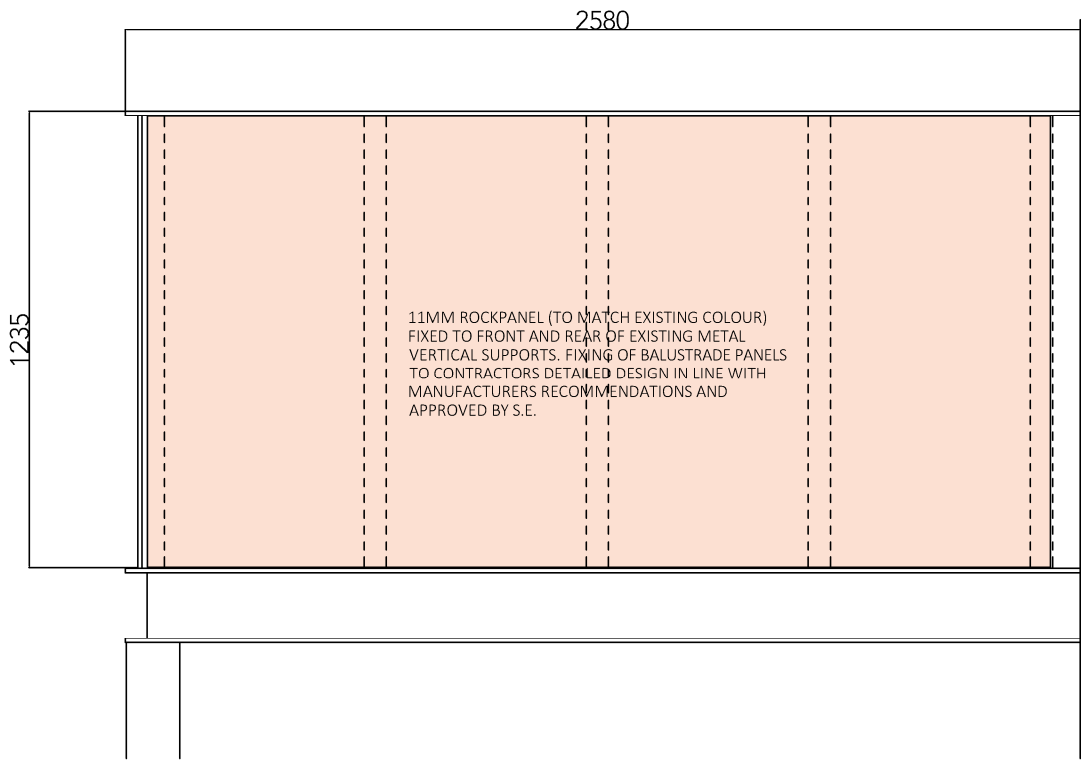
01. FRONT ELEVATION
