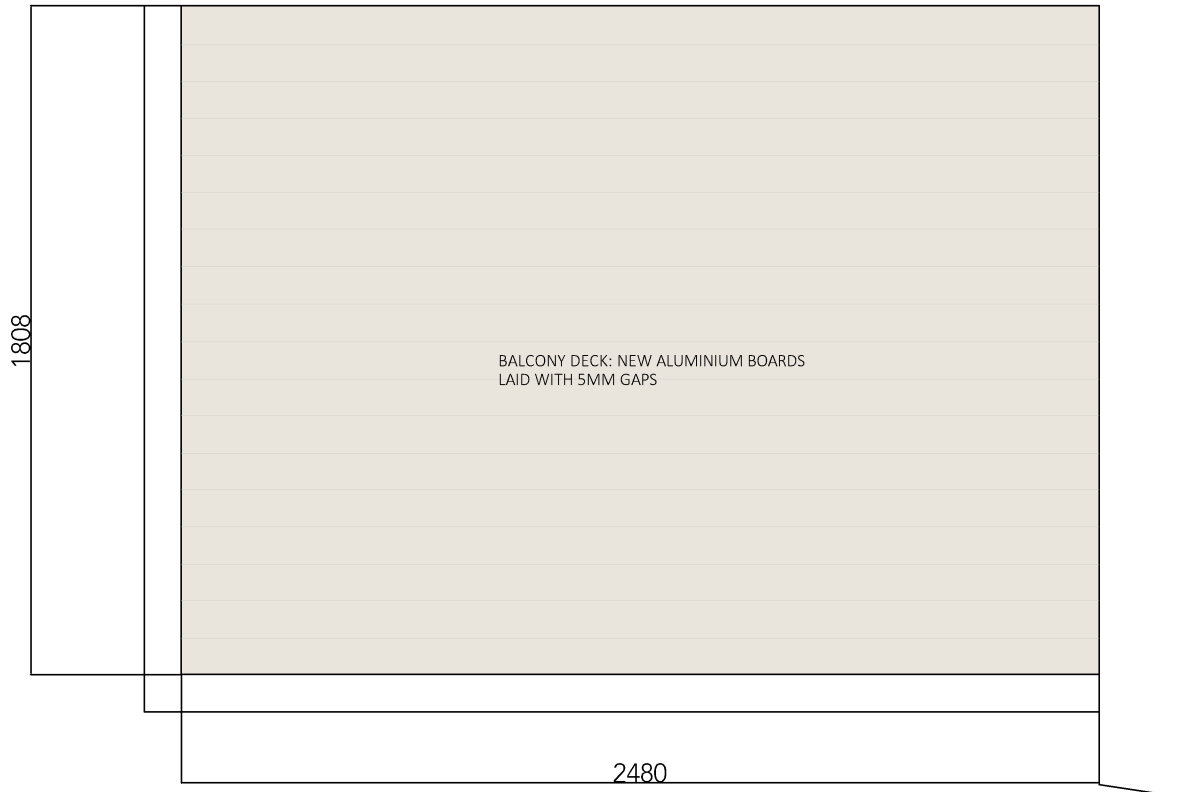
03. PLAN VIEW
