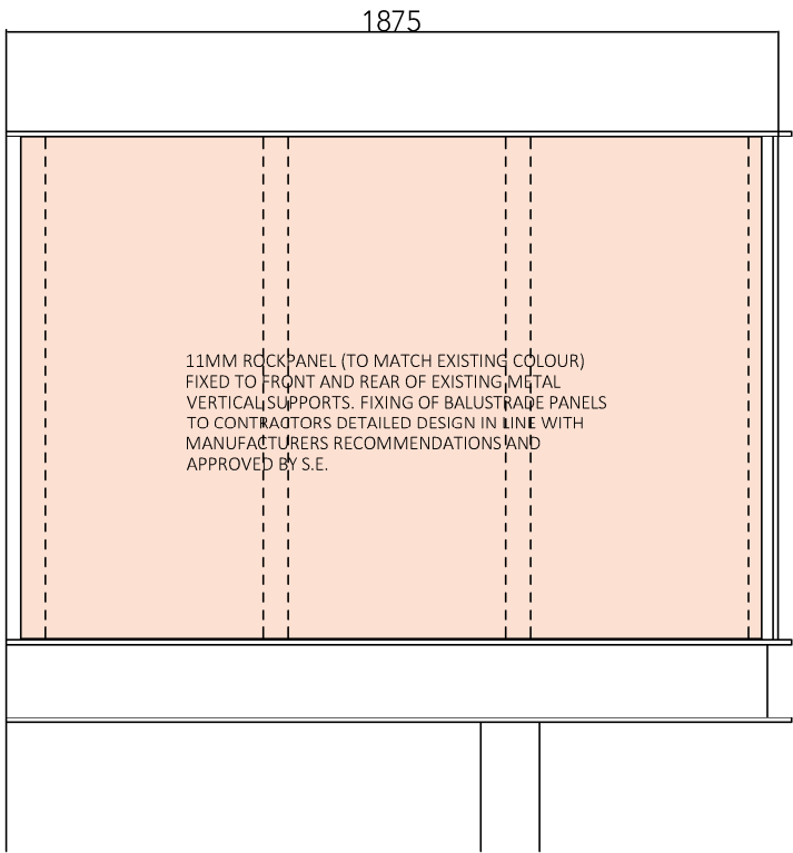
02. SIDE ELEVATION
