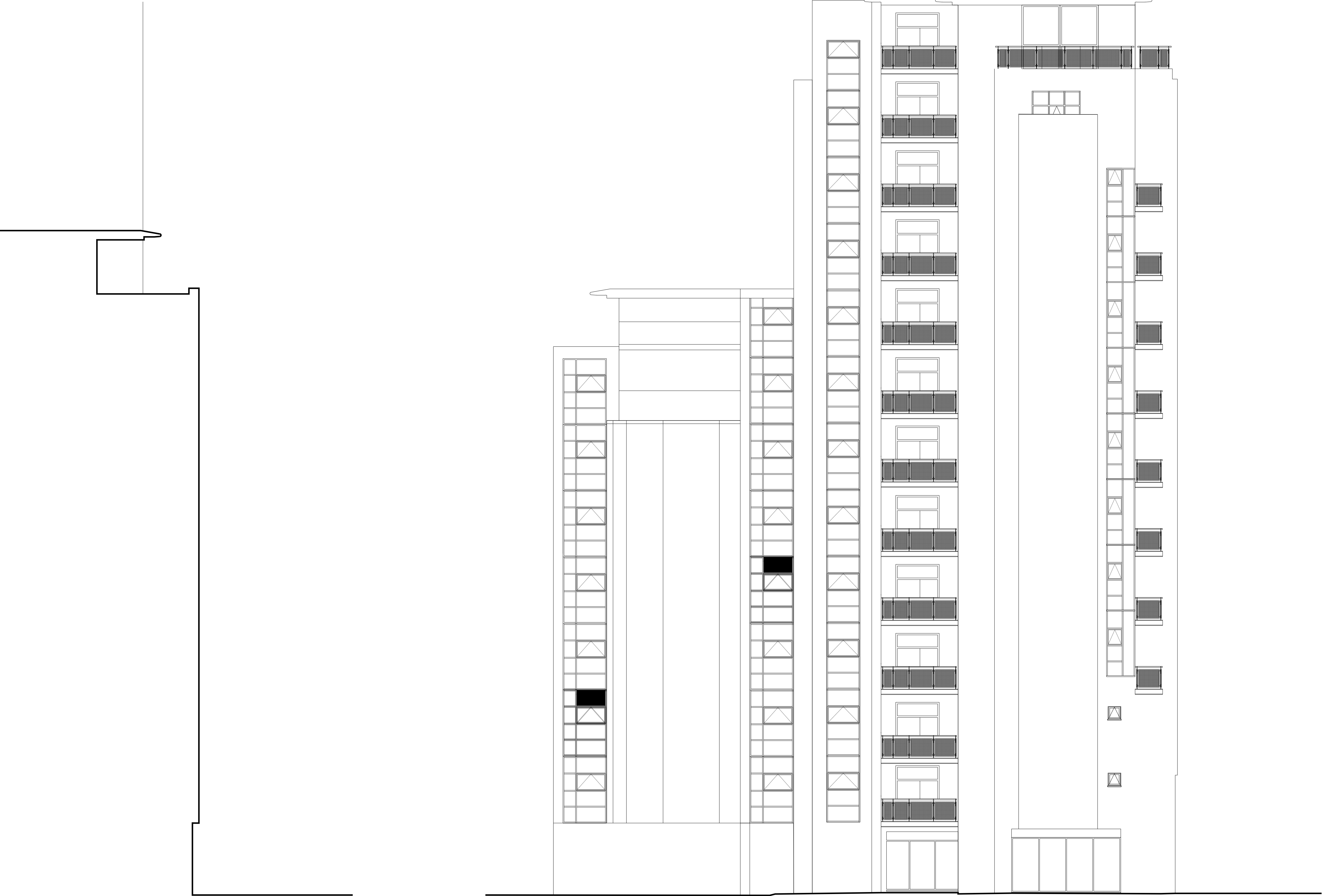
Typical Section Through (as Existing)
