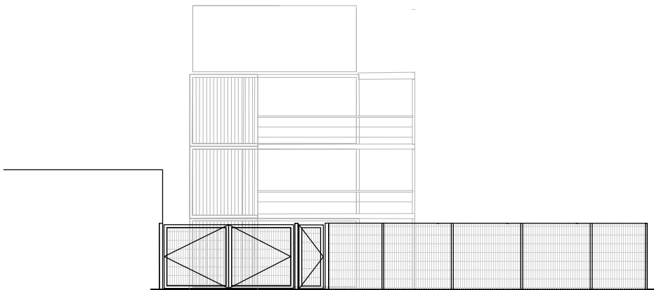
Proposed East Elevation from Manor Street
