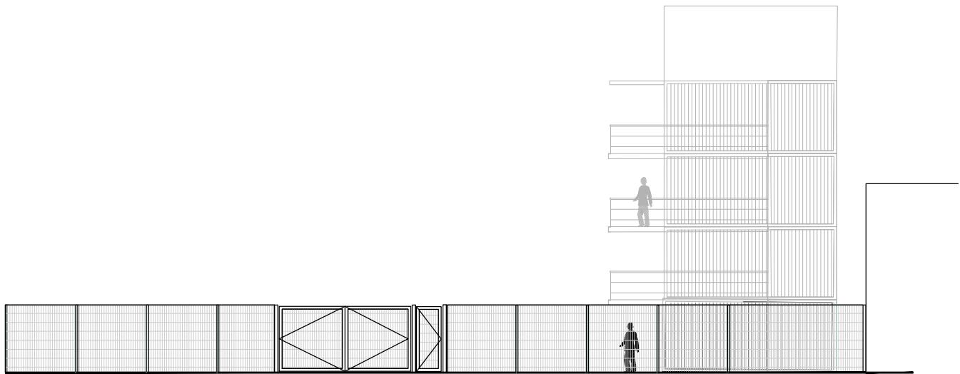
Proposed West Elevation from Cakebread Street
