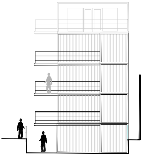
Proposed West Elevation
