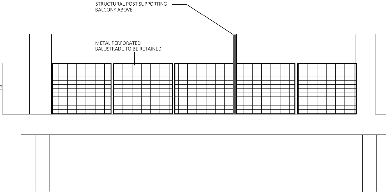
01. FRONT ELEVATION
