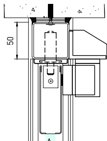
02 MAG-LOCK SCALE 1:5
