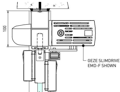
04 AUTOMATIC OVERHEAD OPENER SCALE 1:5
