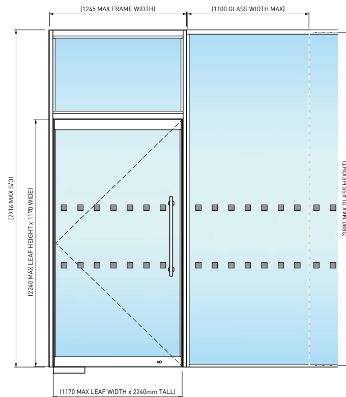
01 MICRO CHANNEL SIDELIGHT - MAX WIDTH SCALE 1:35
