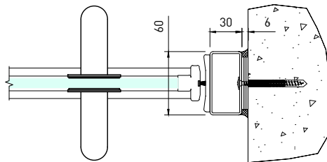
09 LEADING EDGE ABUTMENT SCALE 1:5
