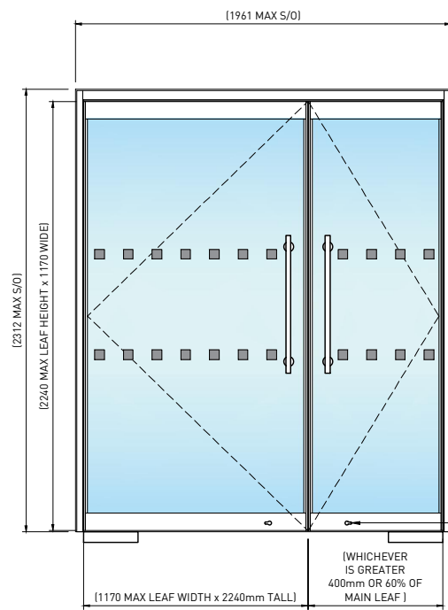
04 HOSPITAL DOORSET - MAX WIDTH SCALE 1:35
