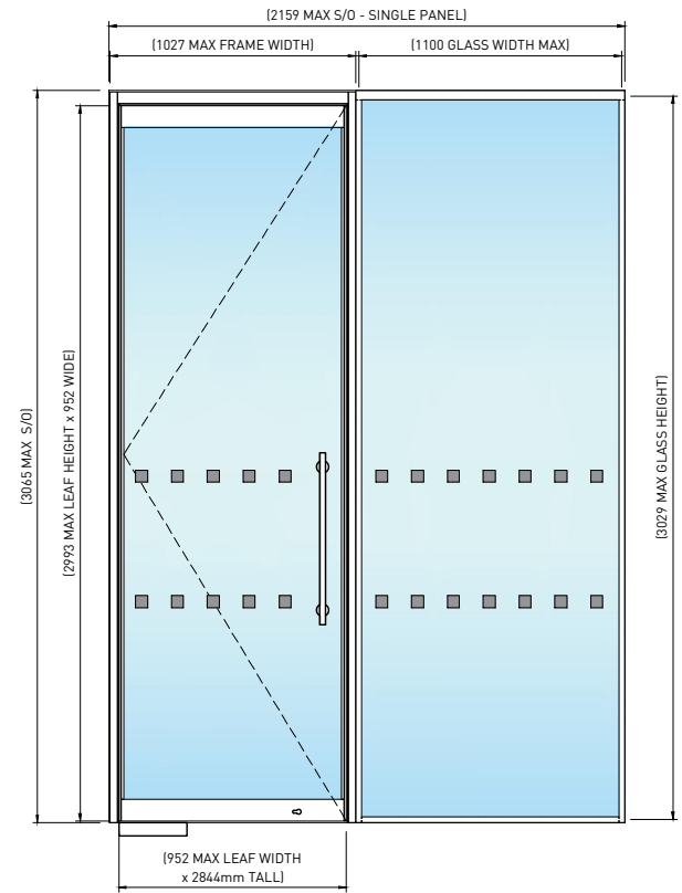
01 MICRO CHANNEL SIDELIGHT - MAX HEIGHT SCALE 1:35
