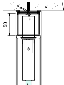
01 CONCEALED SHEARLOCK SCALE 1:5
