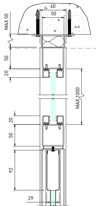
07 OVERPANEL WITH SPIGOTS ABOVE CEILING SCALE 1:5
