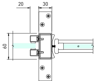
05 PIVOT SIDE WITH BOX & BEAD SCALE 1:5
