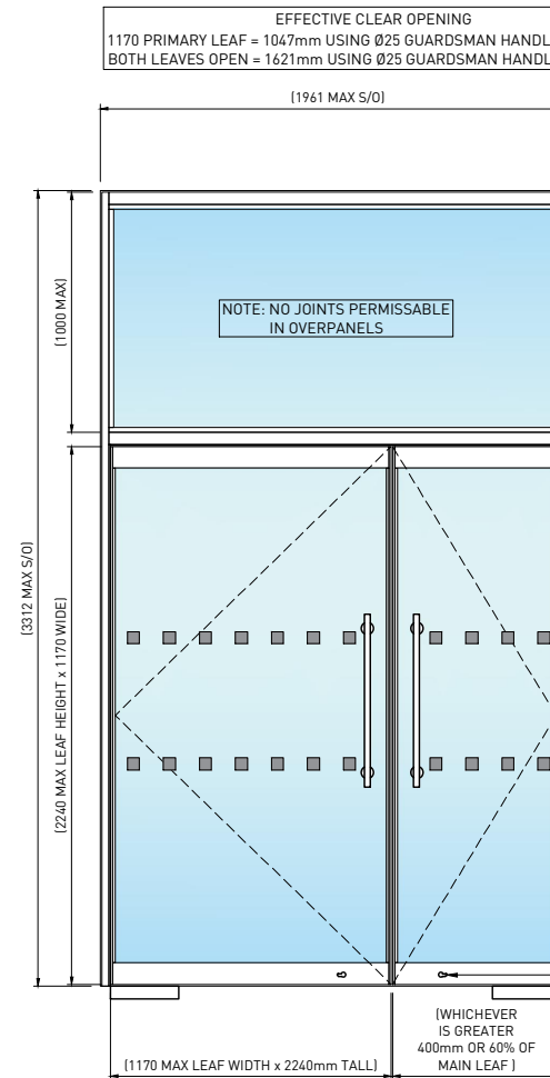
04 HOSPITAL DOORSET - MAX WIDTH SCALE 1:35
