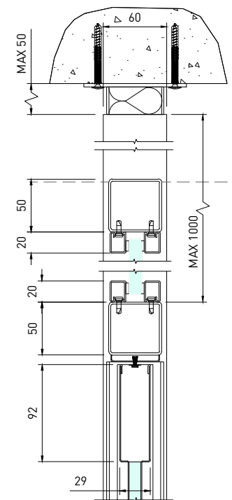
08 OVERPANEL WITH EXTENDED LEGS ABOVE CEILING SCALE 1:5
