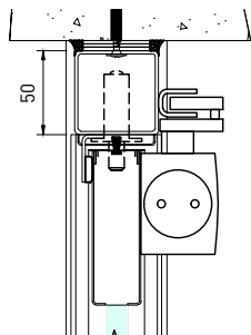
03 OVERHEAD CLOSER SCALE 1:5
