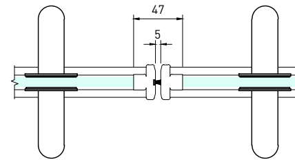
10 DOUBLE DOOR MEETING STILES SCALE 1:5
