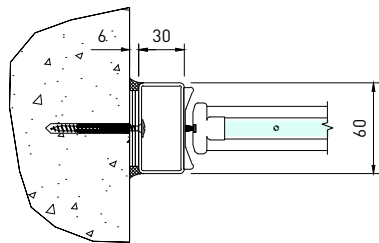
08 PIVOT SIDE ABUTMENT SCALE 1:5
