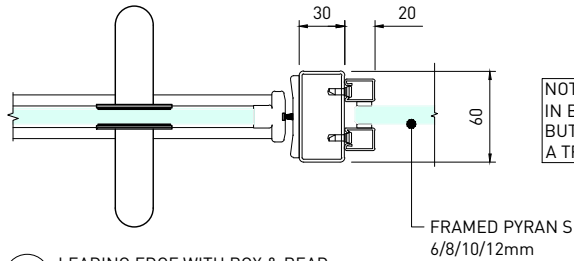
06 LEADING EDGE WITH BOX & BEAD SCALE 1:5
