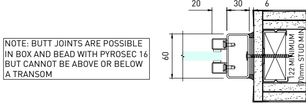
07 BOX & BEAD ABUTMENT SCALE 1:5
