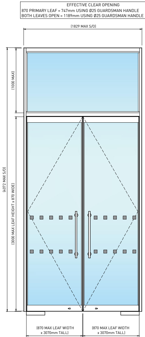
01 DOUBLE DOORSET - MAX HEIGHT SCALE 1:35
