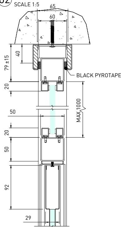
06 OVERPANEL WITH DEFLECTION HEAD SCALE 1:5
