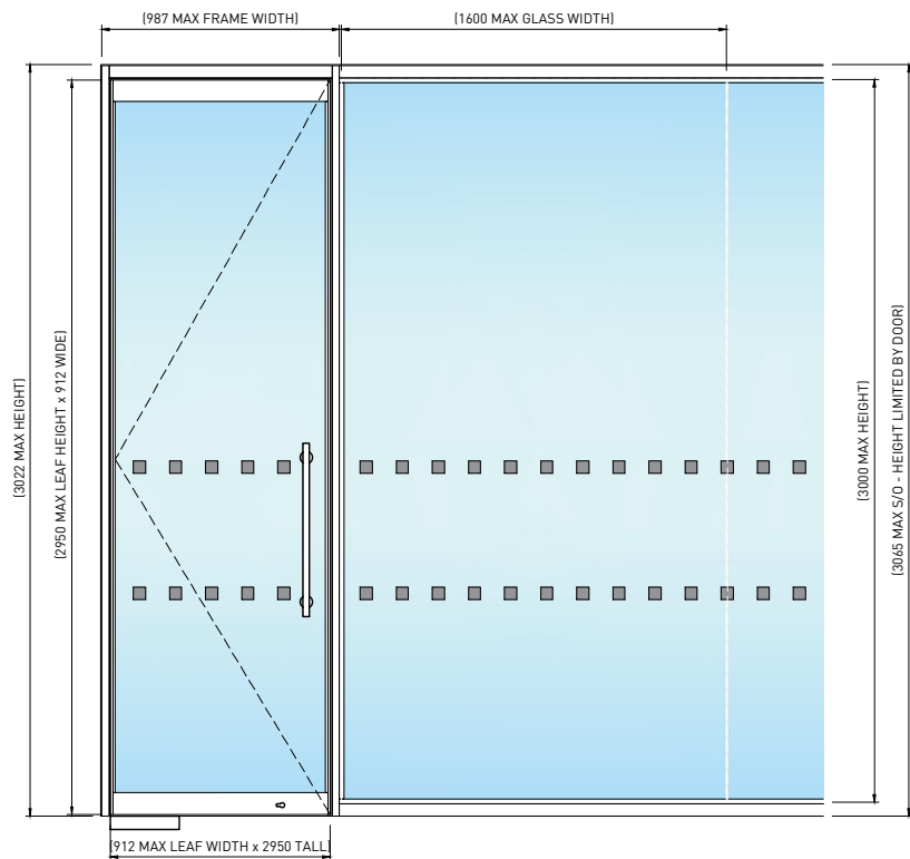
01 BOX & BEAD BUTT JOINTED GLAZING - DOOR MAX HEIGHT SCALE 1:35
