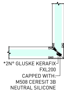
07 MICRO CHANNEL 90° CORNER SCALE 1:5
