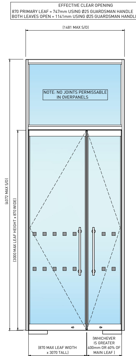
03 HOSPITAL DOORSET - MAX HEIGHT SCALE 1:35
