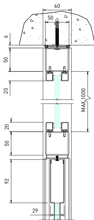
05 OVERPANEL SCALE 1:5
