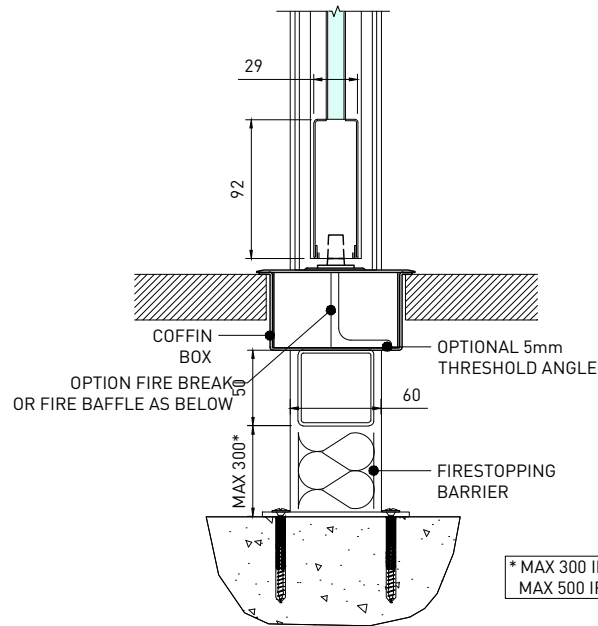
02 FRAMEWORK TO SLAB SCALE 1:5
