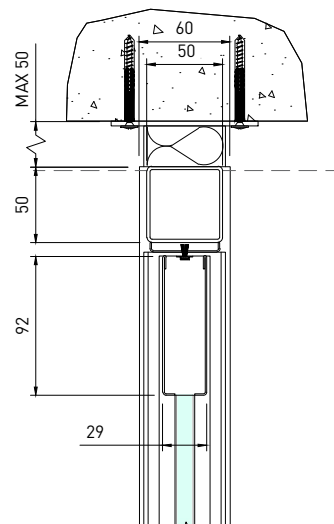
03 SPIGOTS ABOVE CEILING SCALE 1:5
