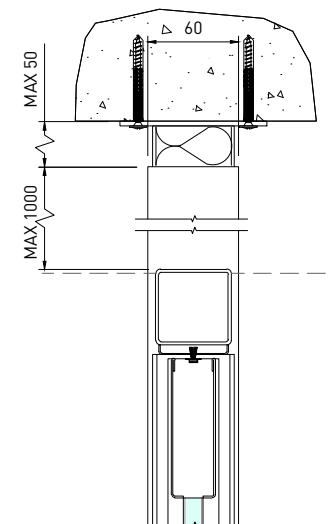
04 DOORFRAME WITH EXTENDED LEGS ABOVE CEILING SCALE 1:5
