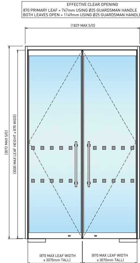
01 DOUBLE DOORSET - MAX HEIGHT SCALE 1:35
