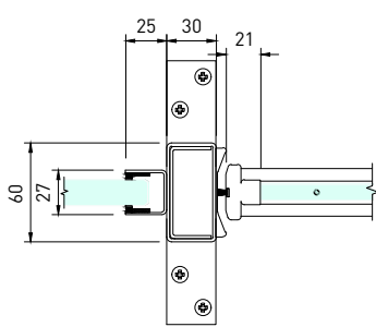
01 PIVOT SIDE MICRO-CHANNEL SCALE 1:5
