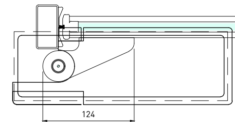
09 OFFSET PIVOT OPTION SCALE 1:5
