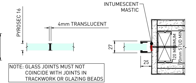
03 PYROSEC GLAZING BUTT-JOINT SCALE 1:5
