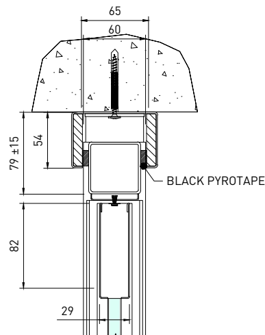
02 DEFLECTION HEAD SCALE 1:5
