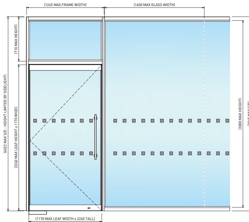
02 BOX & BEAD BUTT JOINTED GLAZING - DOOR MAX WIDTH SCALE 1:35
