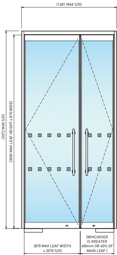
03 HOSPITAL DOORSET - MAX HEIGHT SCALE 1:35
