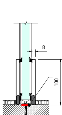
05 GLAZING SKIRTING SCALE 1:5
