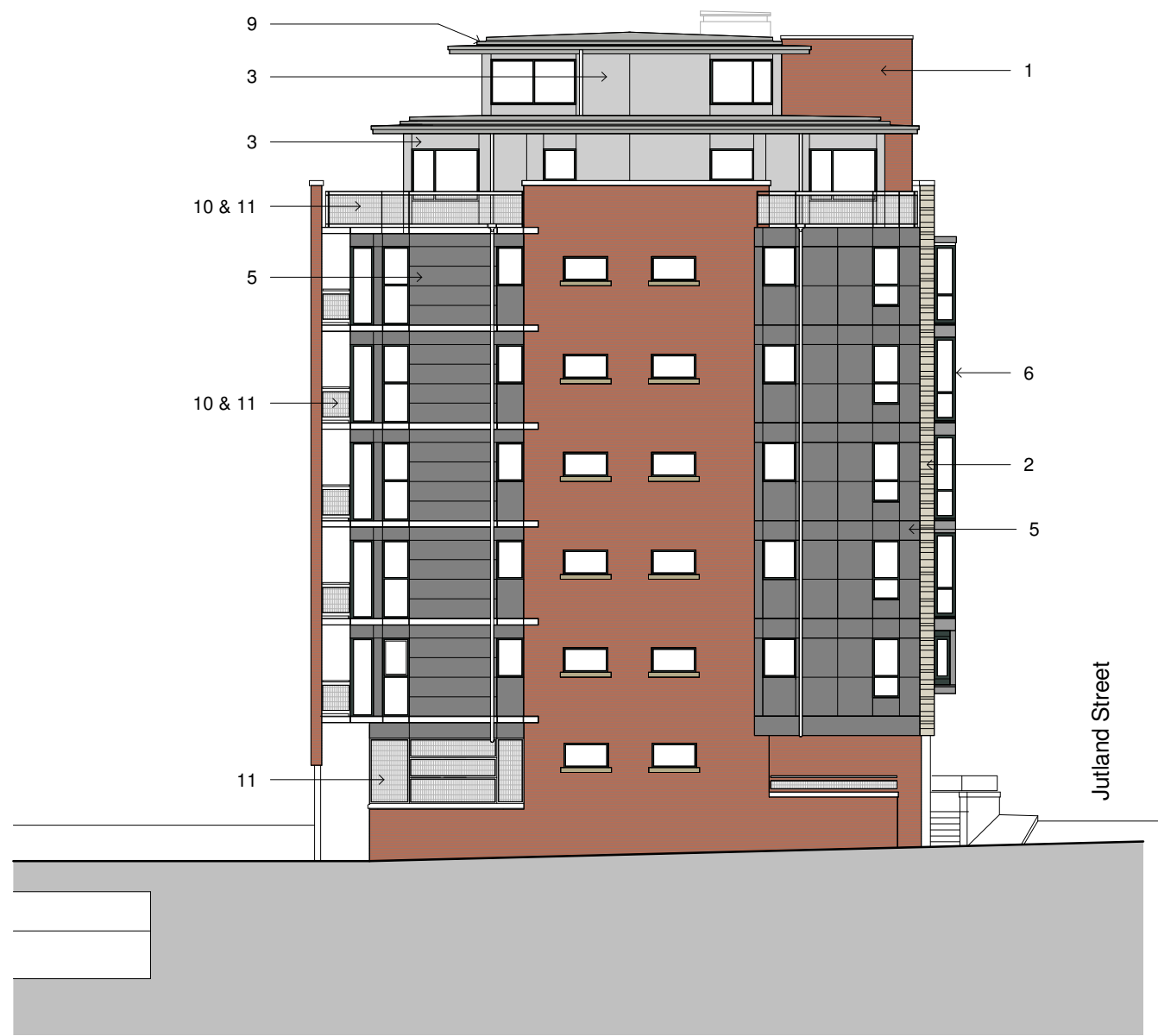
① Jutland House-NW Elevation (Ducie Street)-Proposed 1 : 200
