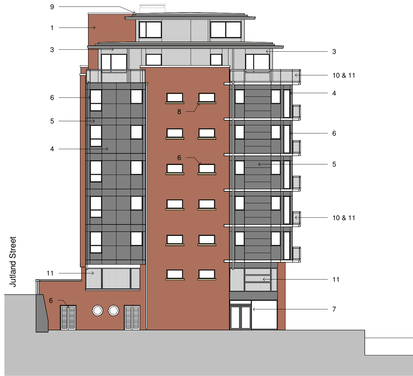
③ Jutland House-SE Elevation (Canal Tow Path)-Proposed 1 : 200
