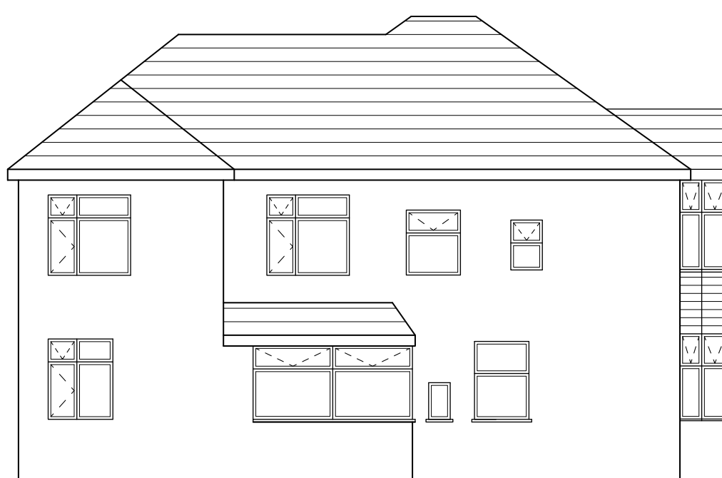
NORTH ELEVATION SCALE 1:100 UID - P008
