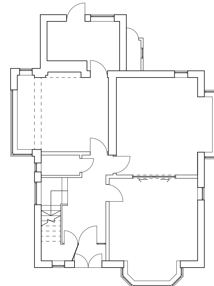
GROUND FLOOR SCALE 1:100 UID - E003
