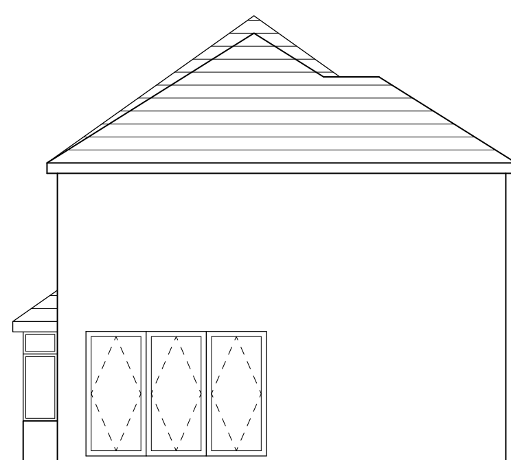
EAST ELEVATION SCALE 1:100 UID - P007
