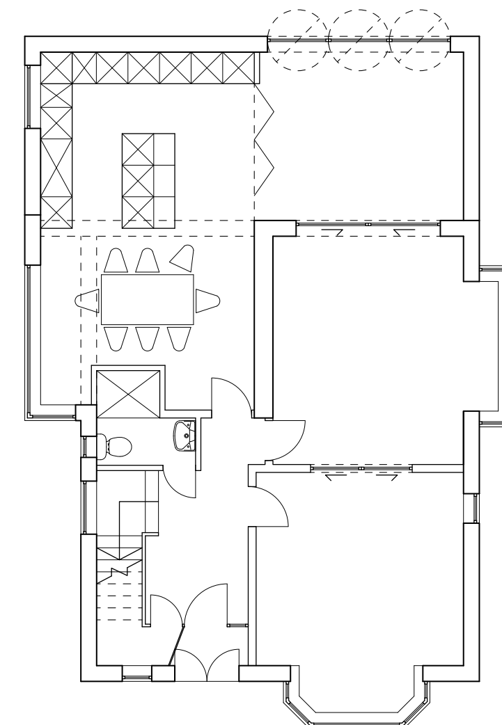
GROUND FLOOR SCALE 1:100 UID - P003
