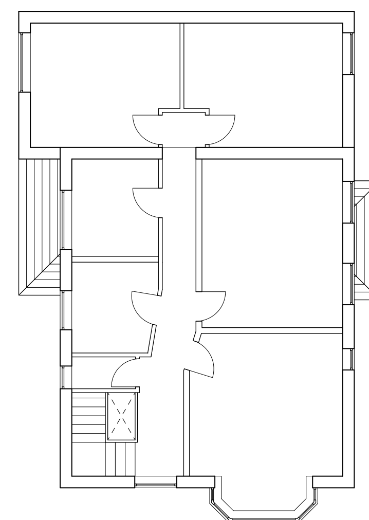
FIRST FLOOR SCALE 1:100 UID - P004
