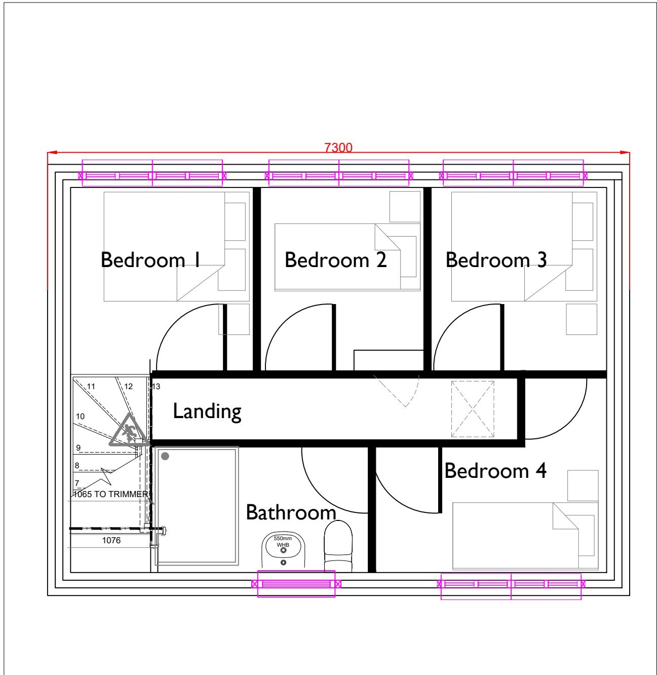
2 EXISTING FIRST FLOOR PLAN 1:50 @ A3
