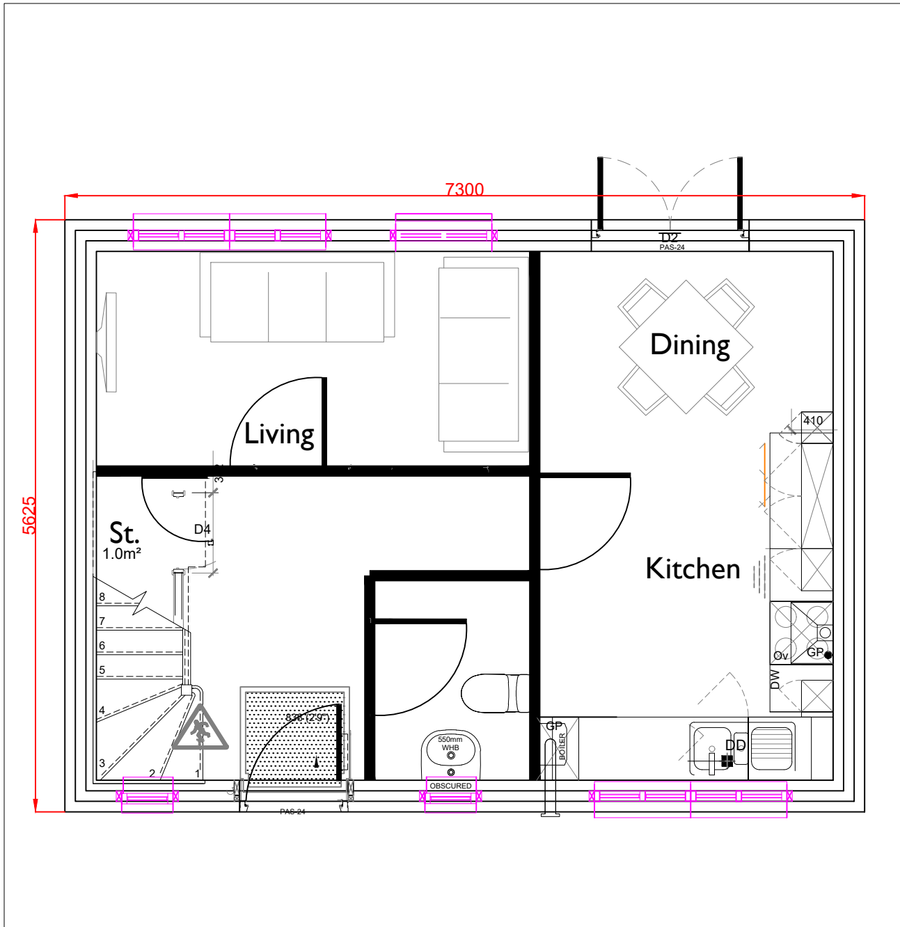
1 EXISTING GROUND FLOOR PLAN 1:50 @ A3
