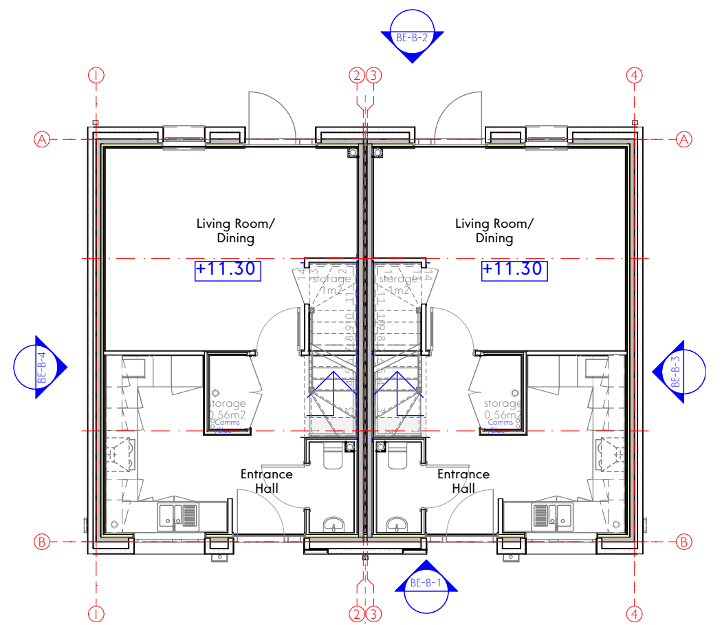
Block G-Ground Floor 2x 2b3p Double Storey Dwellings
