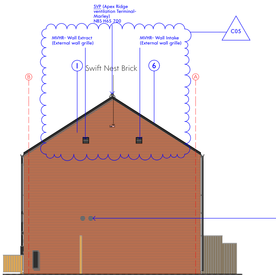
Block G- Elevation E-G-3
