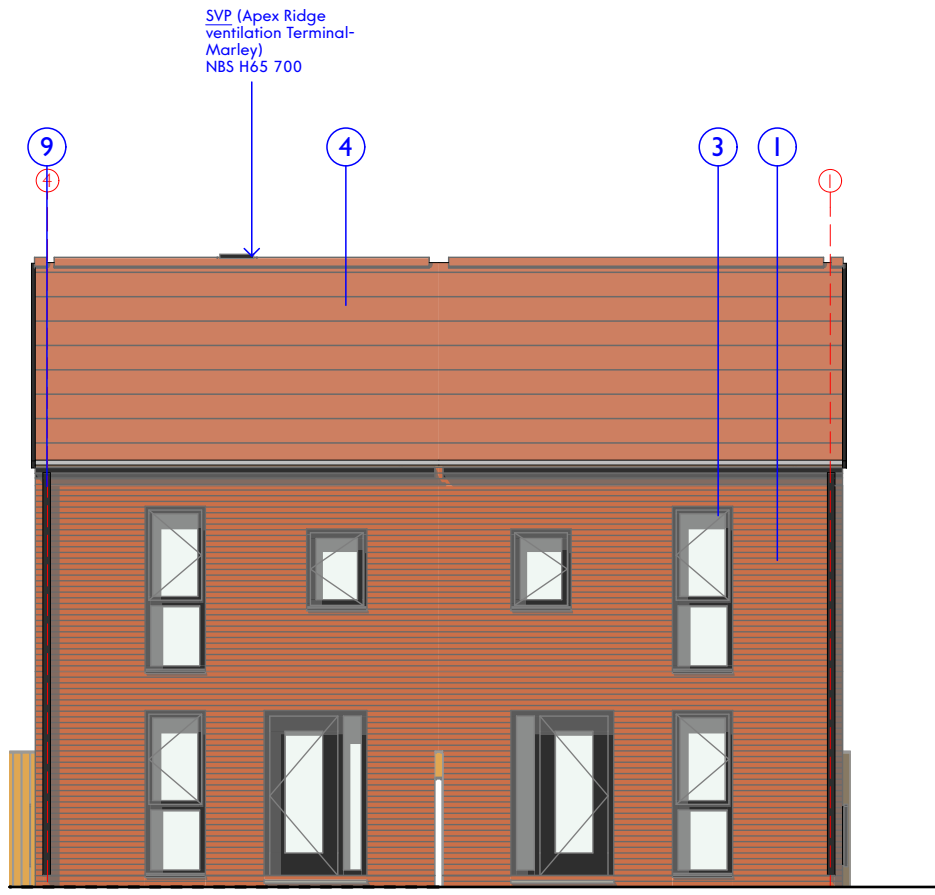
Block G- Elevation E-G-2
