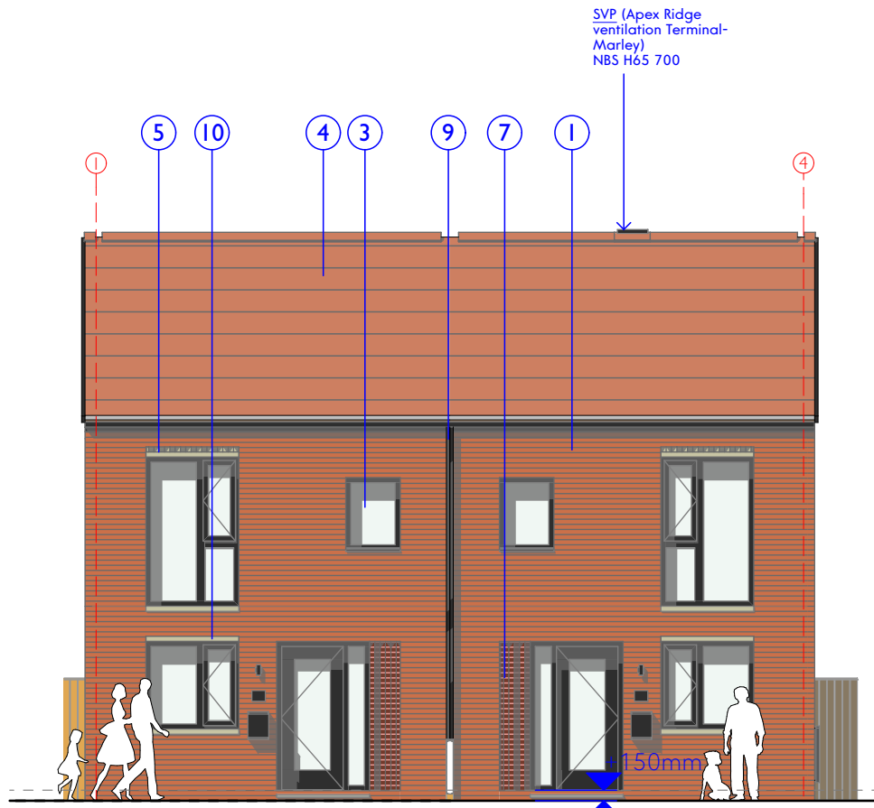
Block G- Elevation E-G-1
