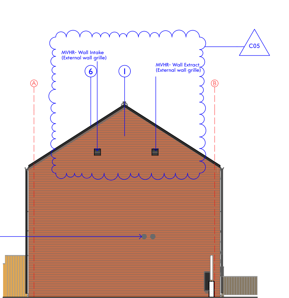
Block G- Elevation E-G-4
