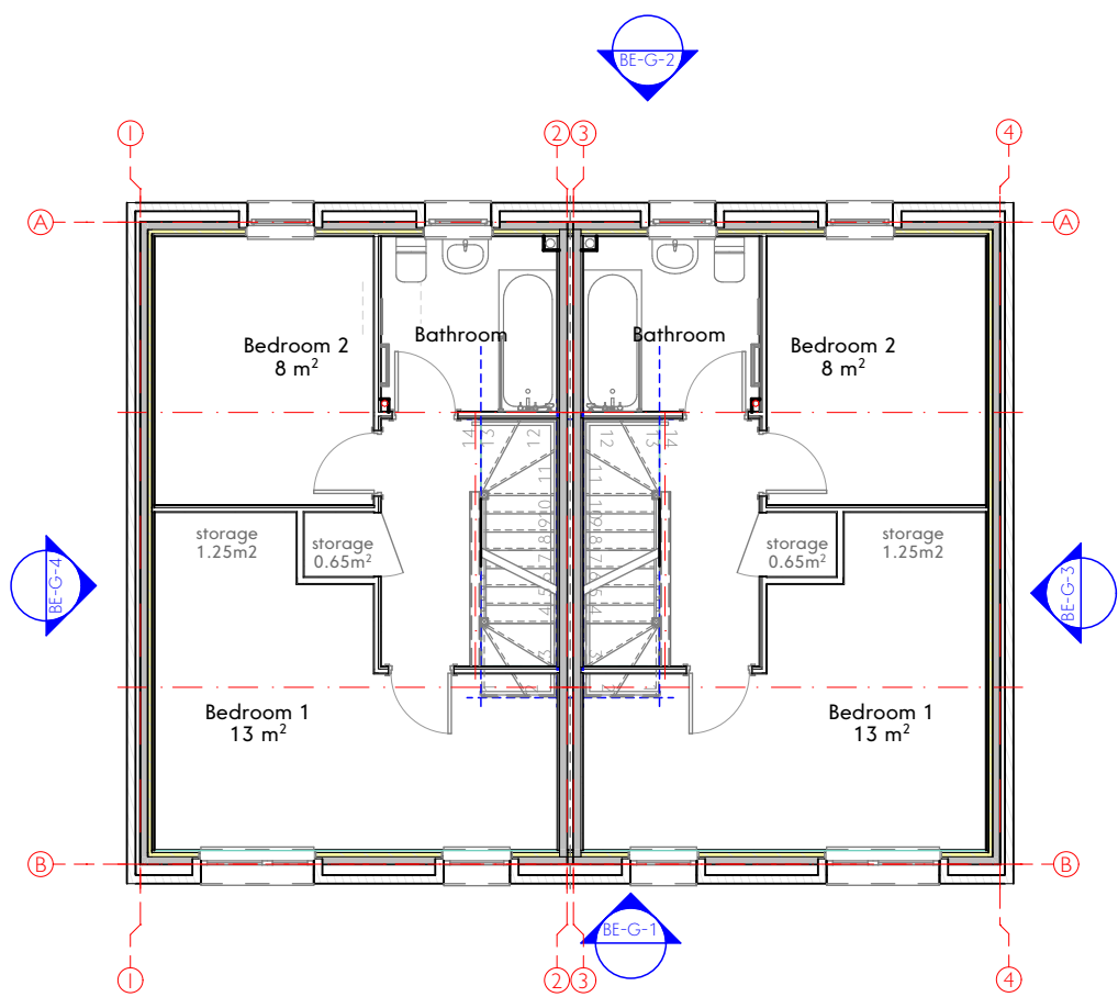
Block G-First Floor 2x 2b3p Double Storey Dwellings
