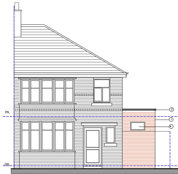
FRONT ELEVATION
