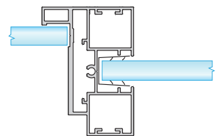
SG DOORSET GLASS (centre)
