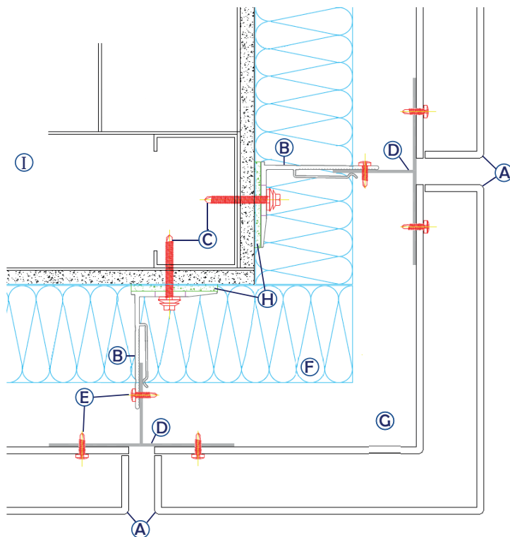
Horizontal Corner Section
